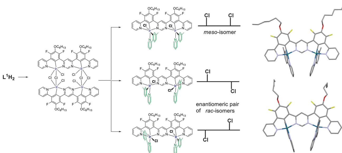
Scheme 2 Synthesis of Ir_2L^1(pty)_2Cl_2 ; schematic illustration of the relative disposition of the Cl ligands (centre), and corresponding structures obtained by X-ray diffraction (right; for clarity, the structures are shown without H atoms, solvent molecules and minor disorder components).
