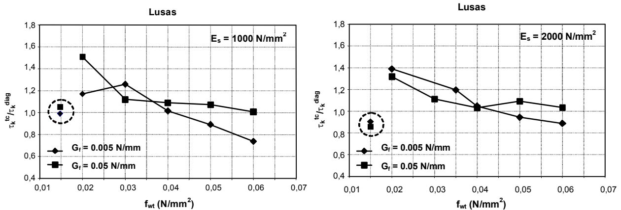
Figs. 8-9 FE Analysis predictions: ratio r = \tau_{0T} / S_S vs. tensile strength of masonry f_{wt} for two values of Young modulus E_s of 1000 MPa and 2000 MPa.
