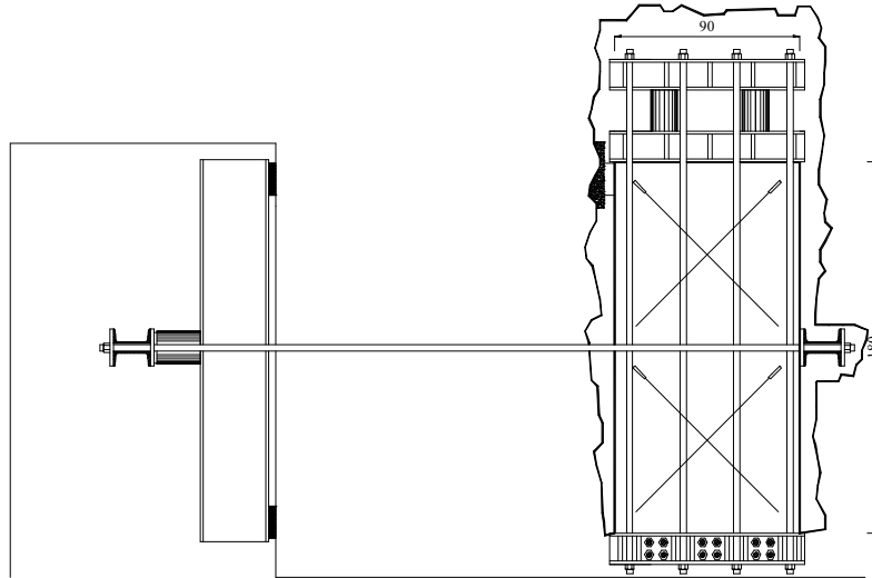
Fig. 2 Position of the inductive transducers during the shear-compression tests on both sides of the masonry panels
