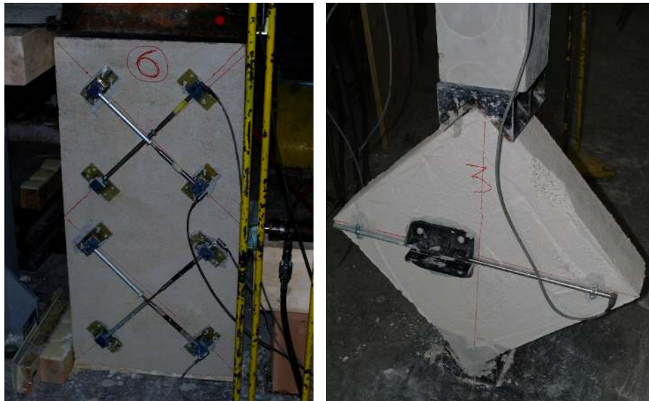
Figs. 5-6 Diagonal compression and shear-compression tests carried out on mortar small-scale panels.
