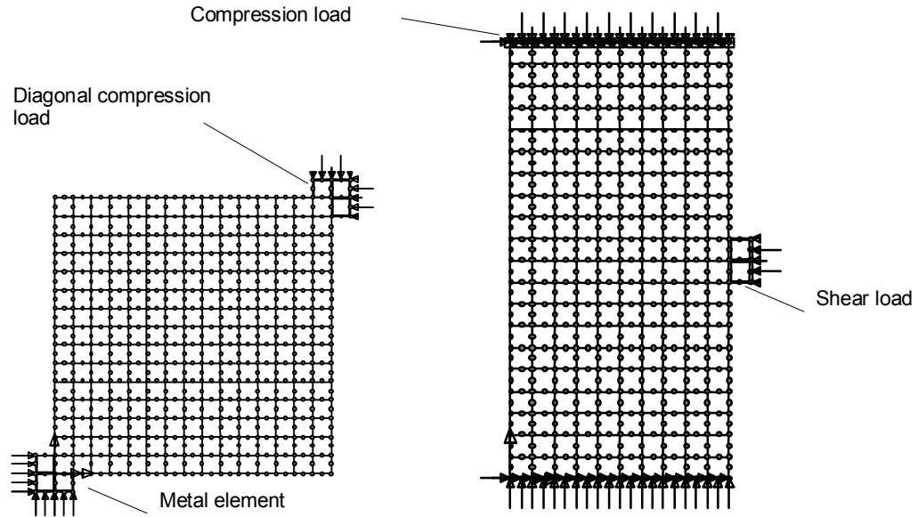
Fig. 7 Modeling of diagonal- and shear-compression tests using the code Lusas.
