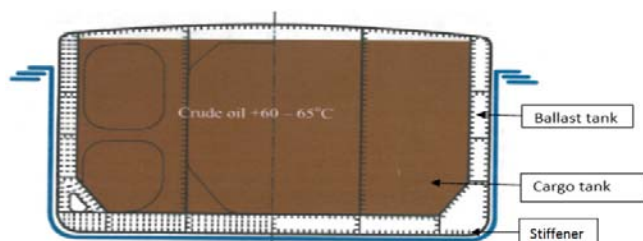
Fig. 2 A ballast tank with stiffeners as compared to a cargo tank in a Crude Oil Carrier
