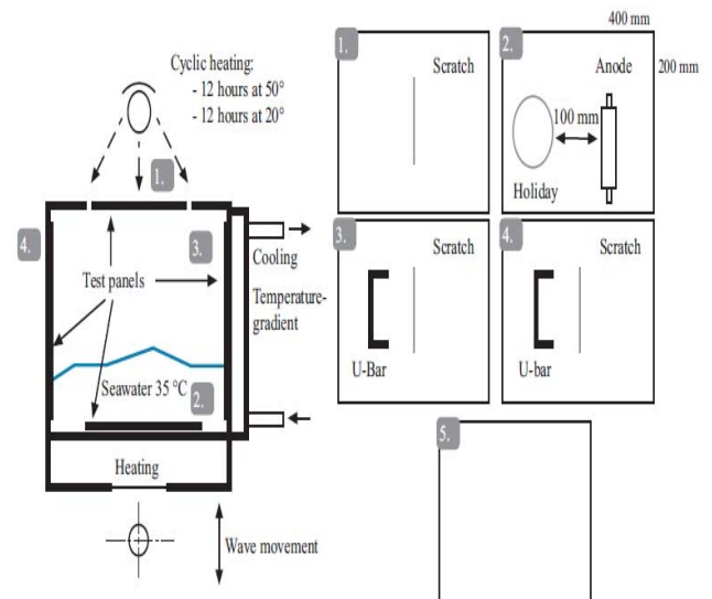
Fig. 3 Wave tank laboratory testing of ballast tank coatings [11]
