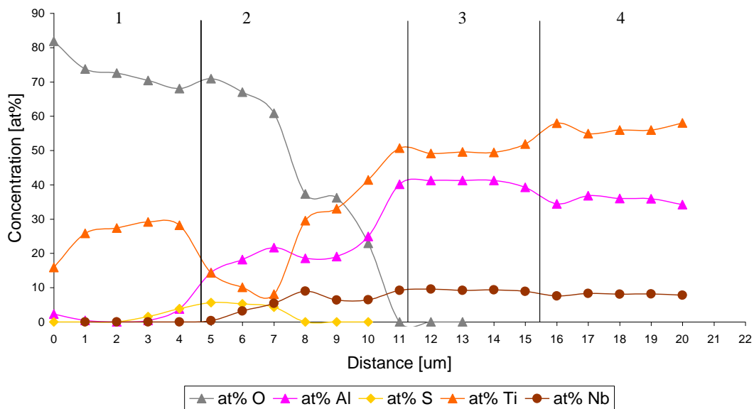
Figure 150 EDS concentration profiles obtained from \text{Ti}_{45}\text{Al}_{18}\text{Nb} uncoated alloy after 1000 hours of sulphidation at 1023 K
