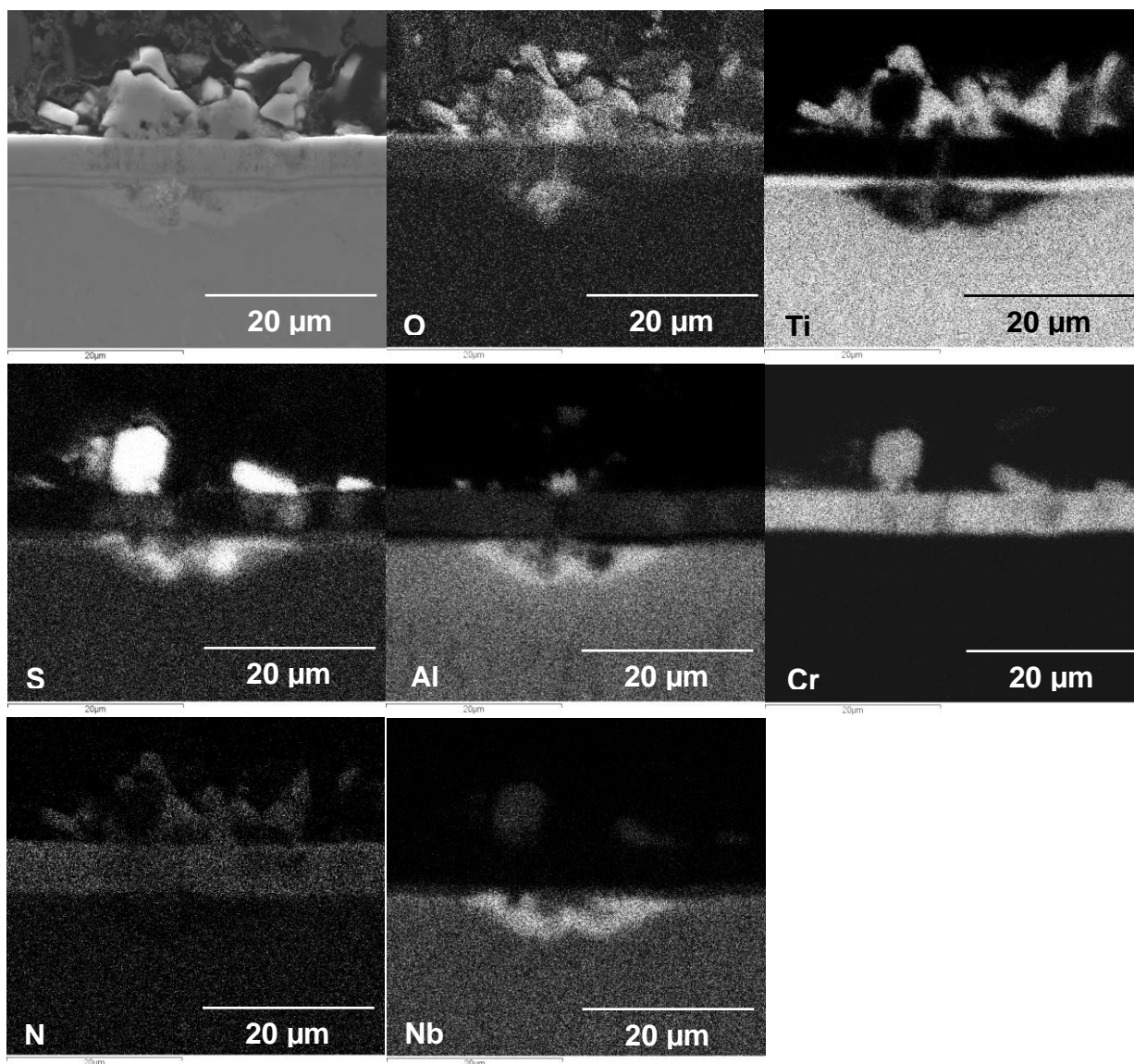
Figure 175 Digimaps of CrAlYN/CrN+CrAlYON coated Ti45Al8Nb etched by CrAl after 1000 hours sulphidation at 1023 K
