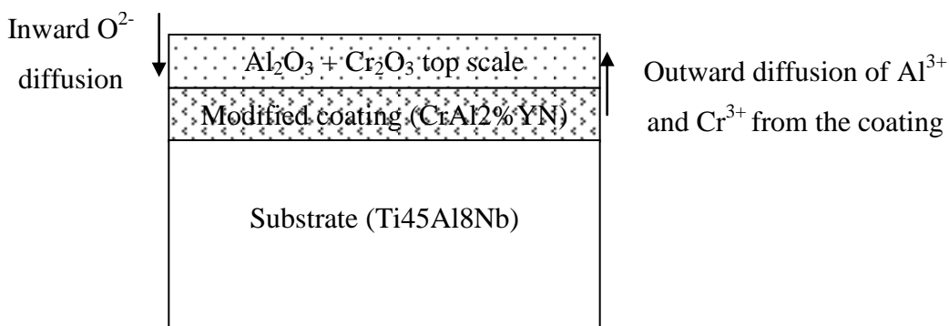
Figure 243 The initial stage of oxidation of CrAl2%YN coated Ti45Al8Nb alloy at 1023 K
