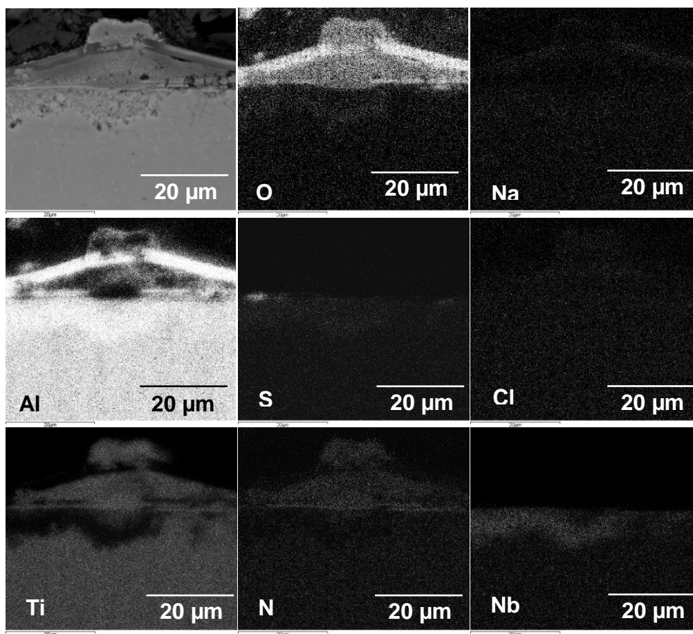
Figure 209 EDS Digimaps of \text{TiAlN} + \text{Al}_2\text{O}_3 top coat coated Ti45Al8Nb after 150 hours hot corrosion exposure at 20%NaCl/80%Na 2 SO 4 salts mixture at 1023 K
