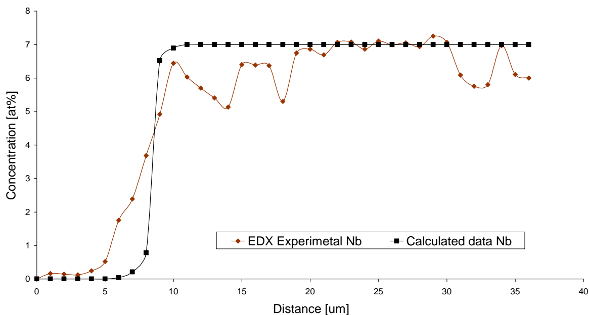
Figure 235 Calculated and experimental concentration profiles for Nb in TiAlCrY coated Ti45Al8Nb after 500 hours at 1123 K in open system (oxidation)
