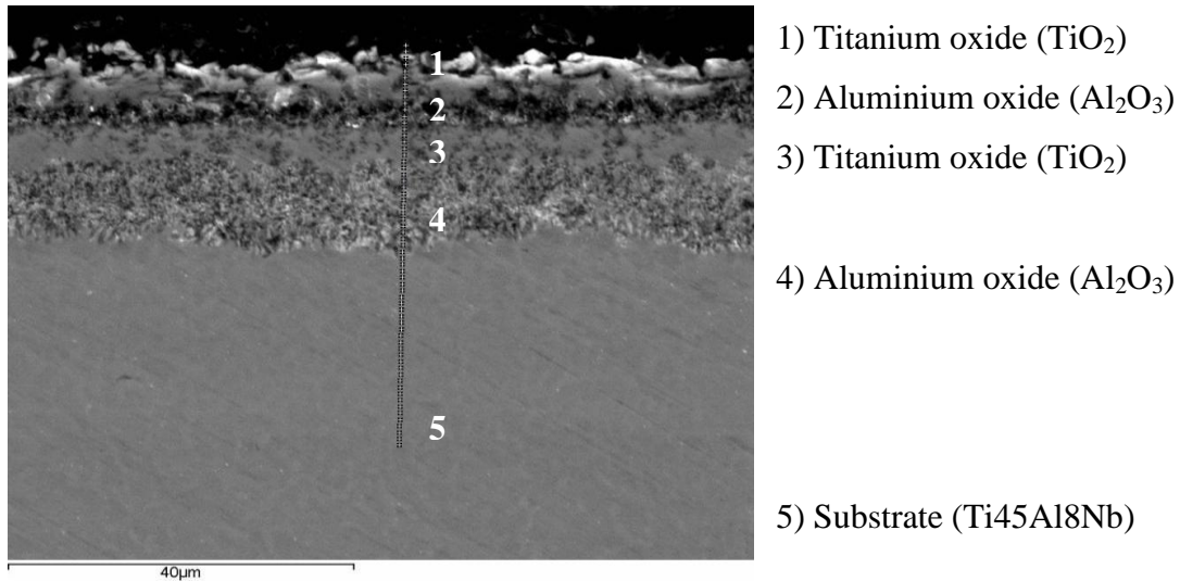
Figure 187 SEM image (mag. 3000x) of base material ( \text{Ti45Al8Nb} ) after 675 hours of sulphidation at 1123 K
