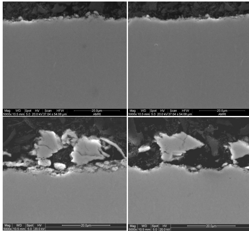
Figure 148 Cross – sectional images of Ti45Al8Nb uncoated sample after 1000 hours sulphidation at 1023 K
