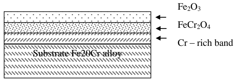
Figure 11 Scale development of oxidized sample in 10%vol. % \text{H}_2\text{O} at 1000 hours for 20 hours [26]
