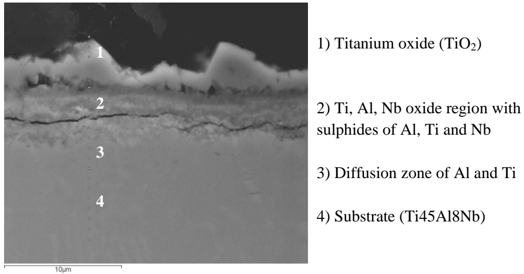
Figure 149 SEM image (mag. 10000x) of base material ( \text{Ti}_{45}\text{Al}_{18}\text{Nb} ) after 1000 hours of sulphidation at 1023 K
