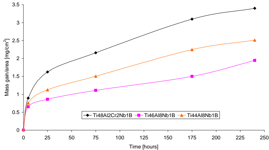
Figure 46 Mass gain of exposed samples to H_2/H_2S/H_2O environments at 1123 K in sulphidation/oxidation test [78]
