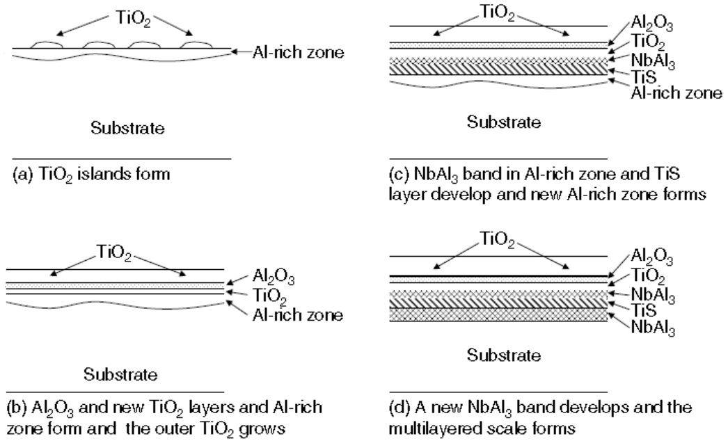
Figure 51 Degradation mechanism for TiAl based intermetallics in H_2/H_2S/H_2O environment at 1123 K [78]
