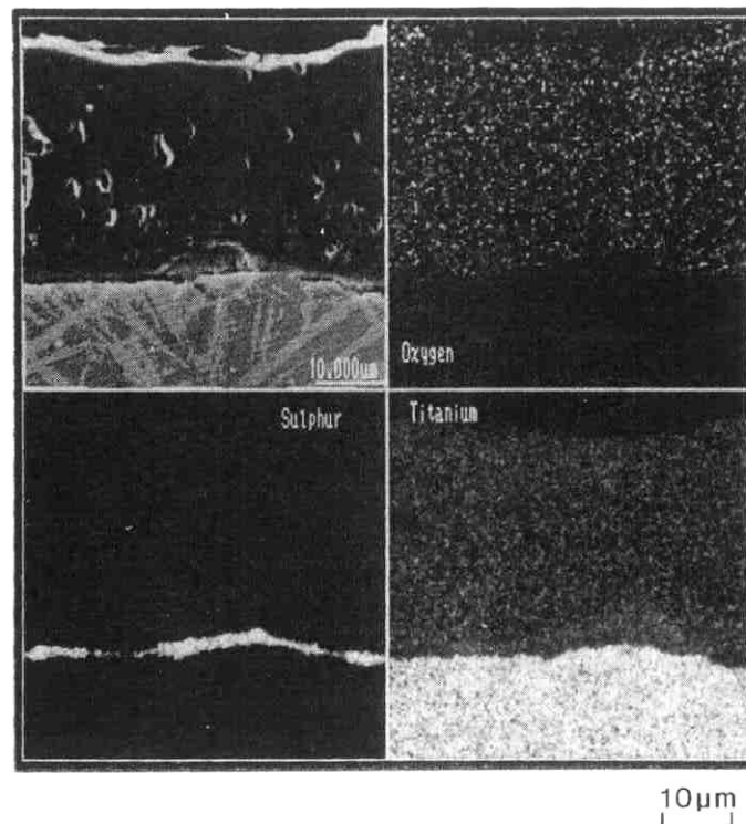
Figure 63 Digimaps of scale morphology on pure Ti after 72 hours at sulphidation oxidation environment ( \text{H}_2/\text{H}_2\text{O}/\text{H}_2\text{S} ) at 1023 K [91]
