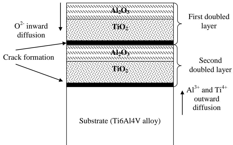
Figure 31d Subsequent \text{Al}_2\text{O}_3 and \text{TiO}_2 layers on Ti6Al4V alloy after oxidation in the temperature range 923 – 1123 K [54]
