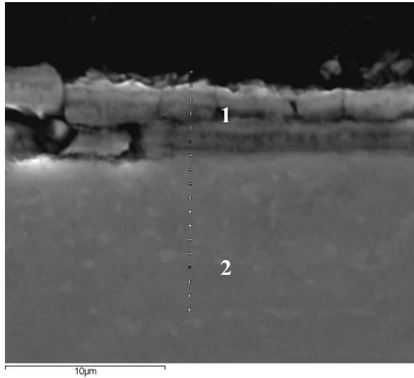
Figure 223 SEM cross section image (mag. 10000x) of TiAlYN/CrN+ \text{Al}_2\text{O}_3 coated Ti45Al8Nb after hot corrosion in salts mixture (20%NaCl/80% \text{Na}_2\text{SO}_4 ) at 1023 K – affected region
