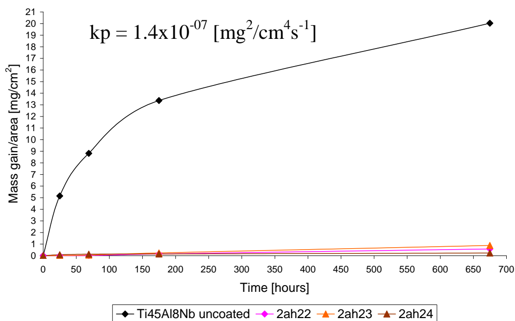
Figure 183 Sulphidation kinetic after 675 hours at 1123 K with k_p value for Ti45Al8Nb alloy
