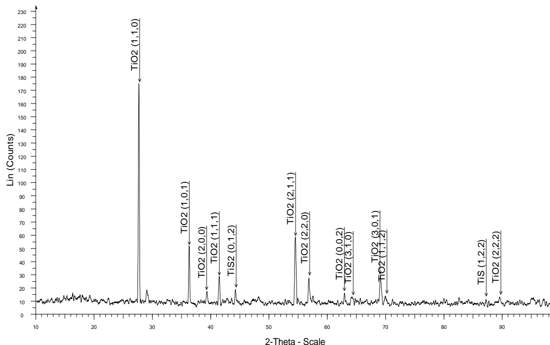
Figure 164 XRD pattern \text{Al}_2\text{Au} coated Ti45Al8Nb after 1000 hours sulphidation at 1023 K
