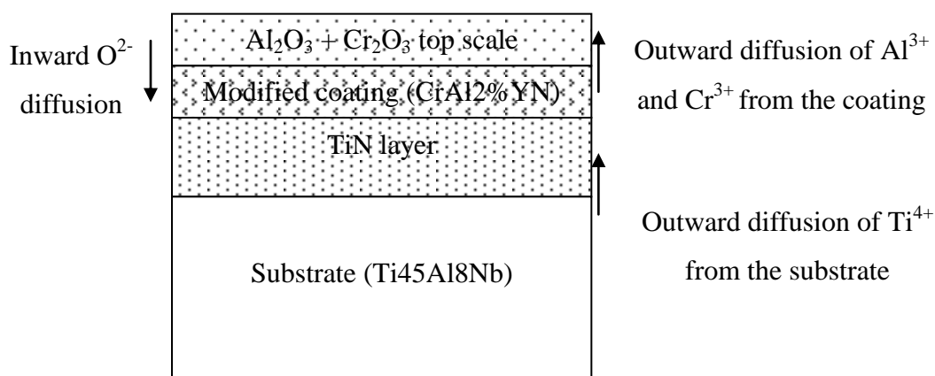
Figure 245 The final scale formed after 500 hours oxidation at 1123 K of CrAl2%YN coated alloy
