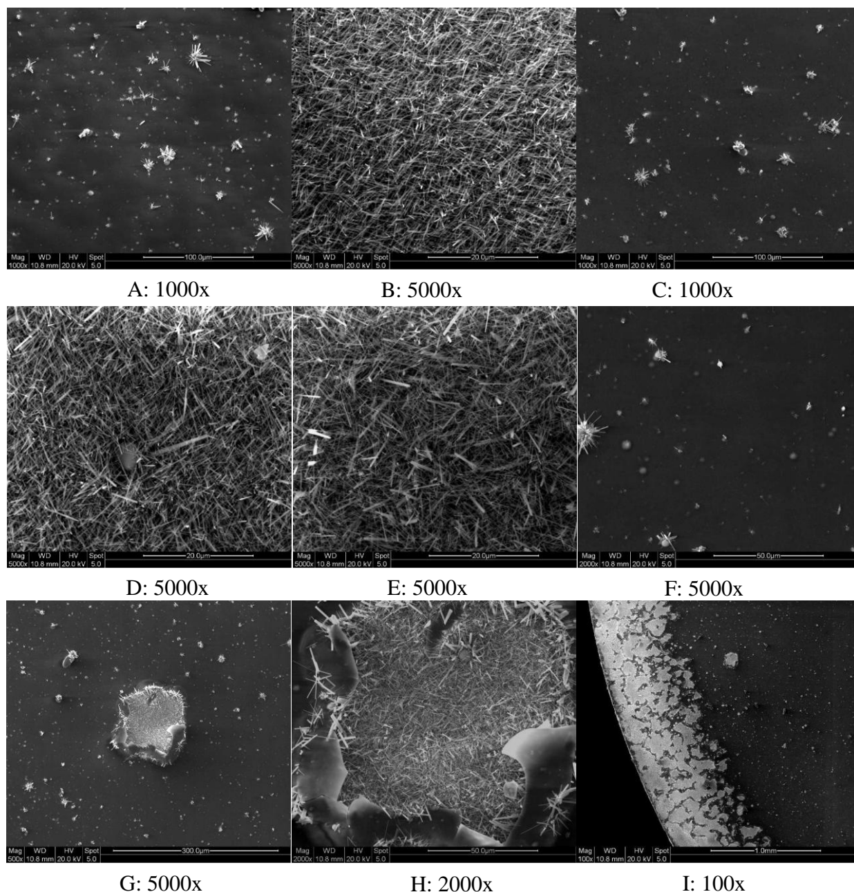
Figure 134 SEM images from surface of TiAlN/CrN+Al 2 O 3 coated Ti45Al8Nb after 5000 hours of oxidation at 1023 K (magnification under images)
