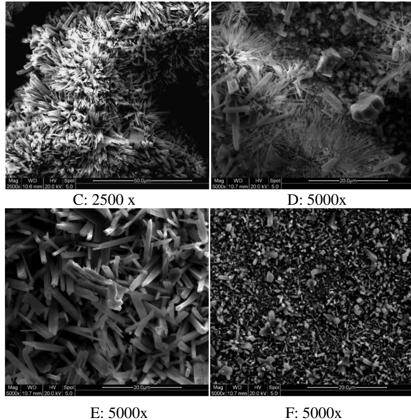
Figure 126 SEM images from surface of TiAlCr coated Ti45Al8Nb after 5000 hours of oxidation at 1023 K (magnification under images)
