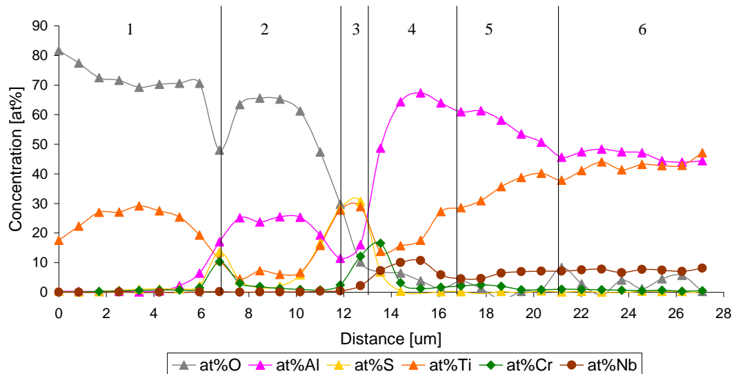
Figure 156 EDS concentration profiles obtained from TiAlCr coated Ti45Al8Nb alloy after 1000 hours of sulphidation at 1023 K
