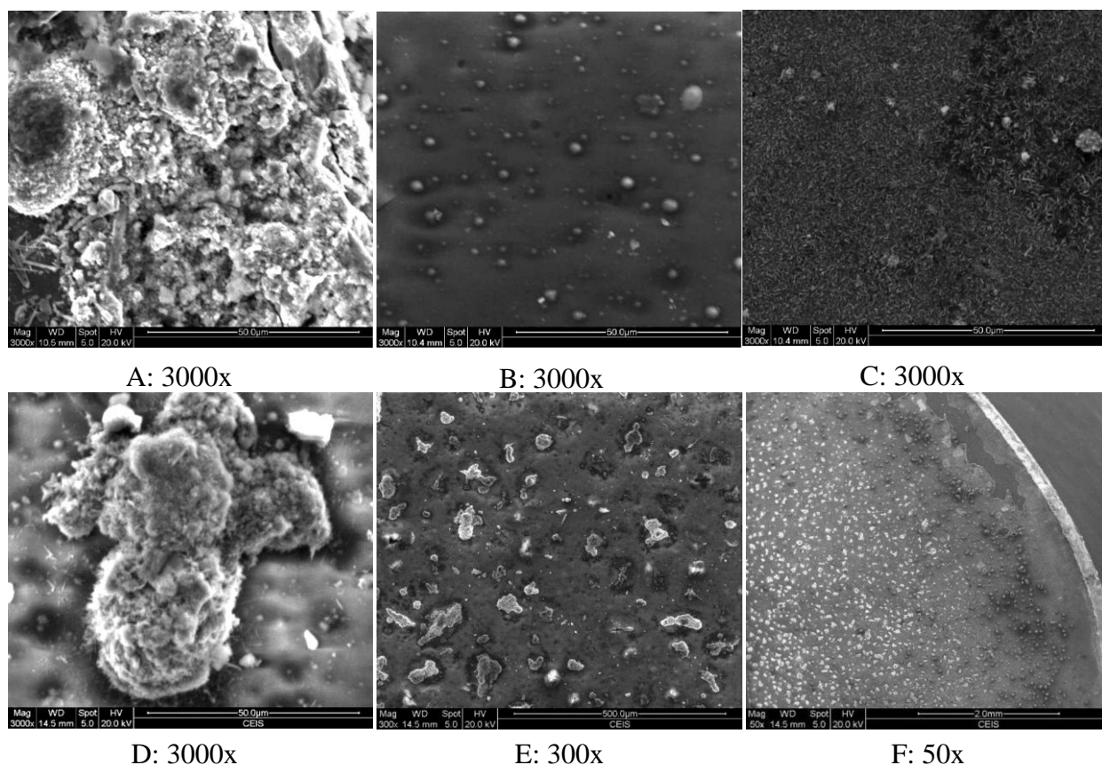
Figure 203 SEM images from surface of TiAlN+Al 2 O 3 coated Ti45Al8Nb after 150 hours hot corrosion/oxidation (20%NaCl/80%Na 2 SO 4 ) at 1023 K (magnification under images)
