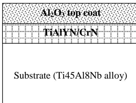
Figure 265 Final stage of exposure of TiAlYN/CrN+Al 2 O 3 coated Ti45Al8Nb alloy during hot corrosion test at 1023 K – unaffected region
