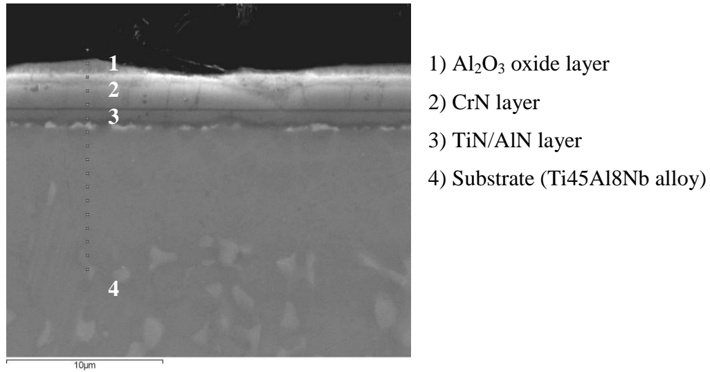
Figure 138 SEM cross section image (mag. 10000x) of the sample ( \text{TiAlYN/CrN}+\text{Al}_2\text{O}_3 coated Ti45Al8Nb after 5000 hours of oxidation at 1023 K with EDS line – picture taken from the middle of the sample
