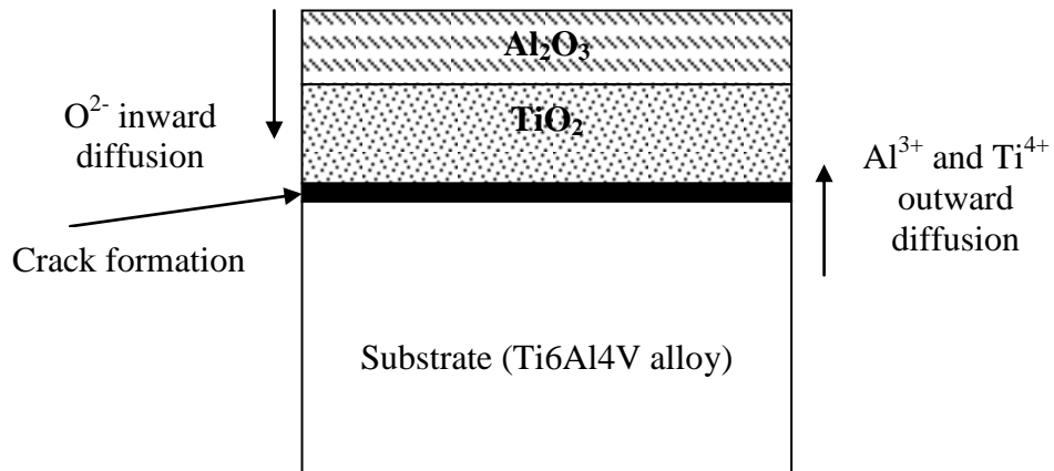
Figure 31c \text{Al}_2\text{O}_3 and the crack formation [54]
