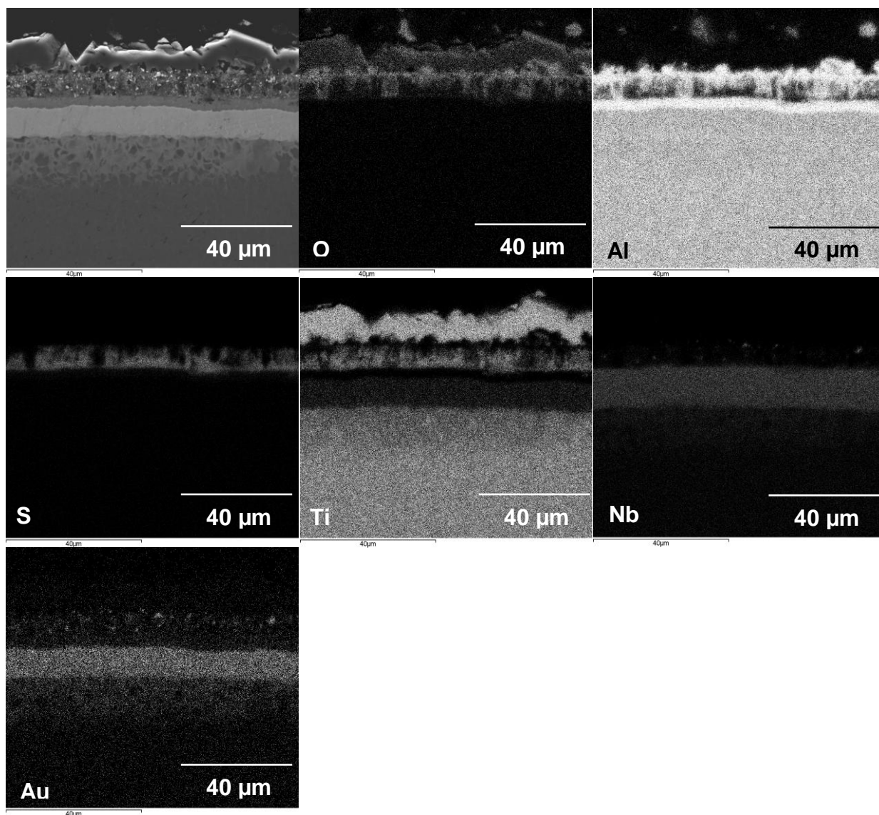
Figure 163 Digimaps of \text{Al}_2\text{Au} coated \text{Ti}_{45}\text{Al}_{8}\text{Nb} after 1000 hours sulphidation at 1023 K
