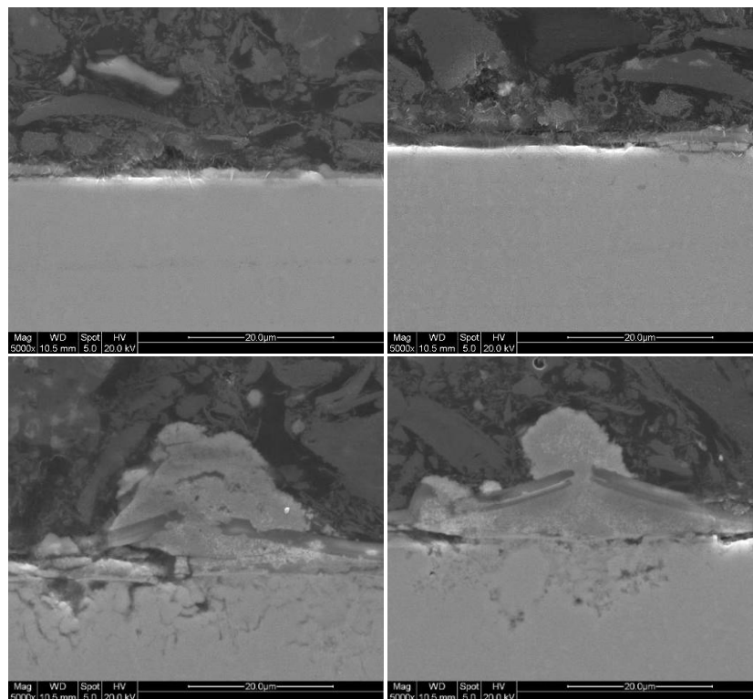
Figure 204 Cross – sectioned images of TiAlN + Al 2 O 3 coated Ti45Al8Nb after hot corrosion in salts mixture (20%NaCl/80%Na 2 SO 4 ) at 1023 K
