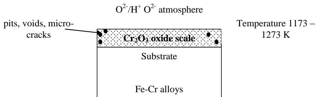
Figure 12a Initial period of oxidation in the wet atmosphere at temperature 1173 – 1273 K of Fe20Cr alloys [26]
