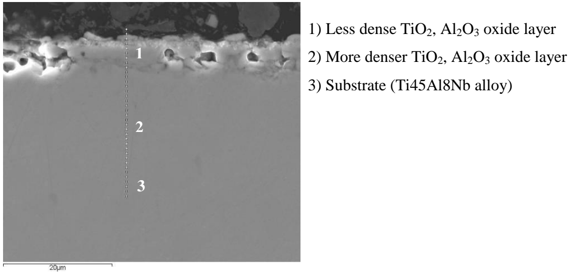
Figure 117 Cross – section SEM image (mag. 5000x) of TiAlCrY coated Ti45Al8Nb alloy after 500 hours of oxidation at 1223 K
