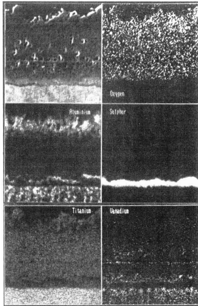
Figure 64 Digimaps of scale morphology of Ti6Al4V alloy after 72 hours at sulphidation oxidation environment ( H_2/H_2O/H_2S ) at 1023 K [91]
