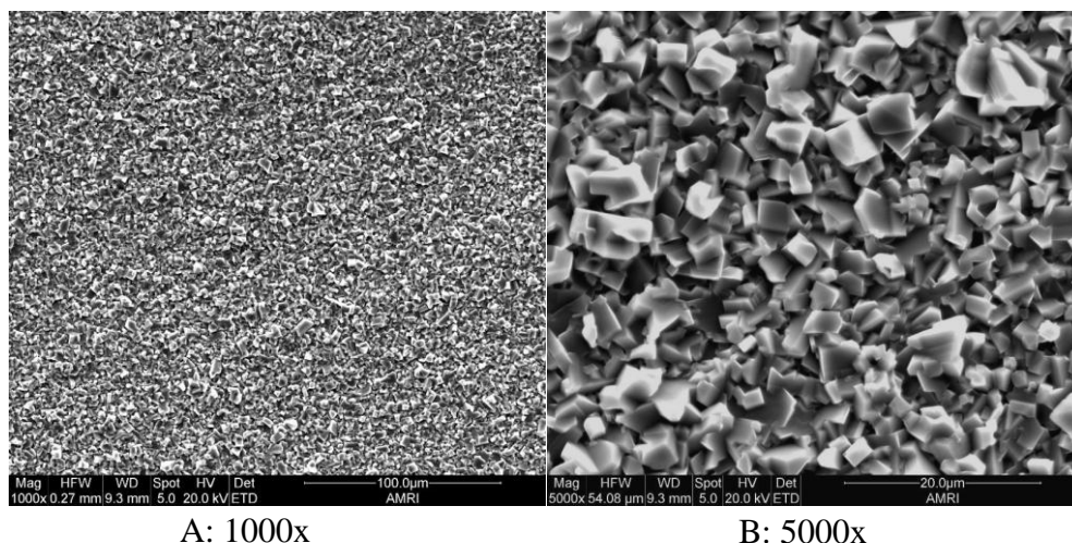
Figure 147 Surface morphology of Ti45Al8Nb uncoated after 1000 hours of sulphidation at 1023 K (magnification under images)
