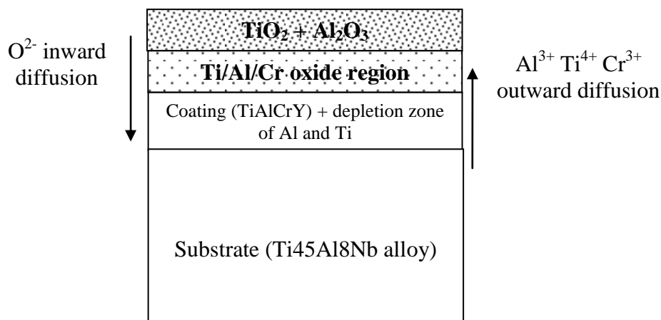
Figure 240 Scale formed in TiAlCrY coated Ti45Al8Nb alloy after 500 hours oxidation at 1123 K
