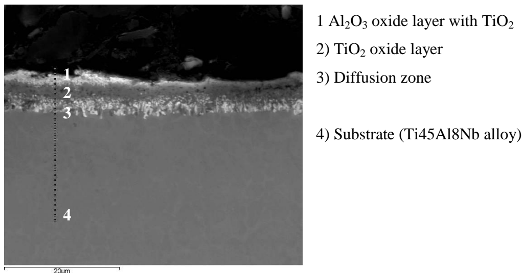
Figure 144 SEM cross section image (mag. 5000x) of the \text{TiAlN}+\text{Al}_2\text{O}_3 coated \text{Ti45Al8Nb} after 5000 hours of oxidation at 1023 K with EDS line – picture taken from middle of the sample
