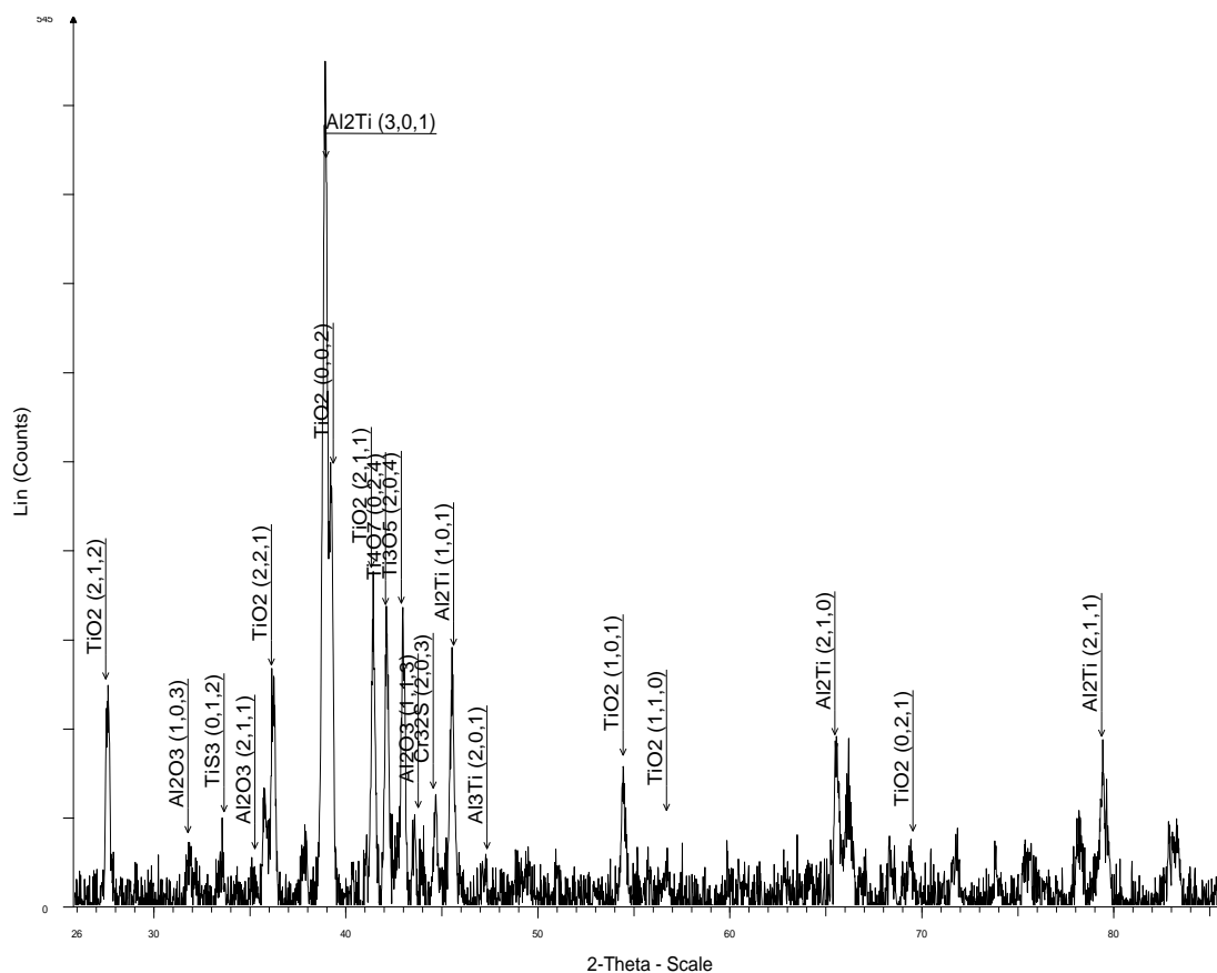
Figure 158 XRD pattern TiAlCr coated Ti45Al8Nb after 1000 hours sulphidation at 1023 K
