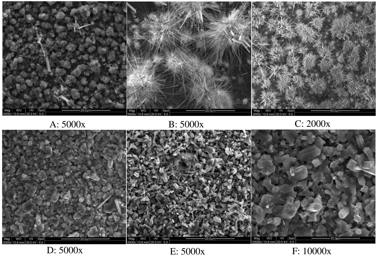
Figure 140 SEM images from surface of TiAlN + Al 2 O 3 coated Ti45Al8Nb after 5000 hours oxidation of oxidation at 1023 K (magnification under images)
