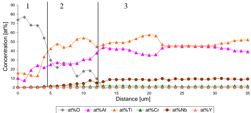
Figure 118 EDS concentration profiles obtained from TiAlCrY coated Ti45Al8Nb alloy after 500 hours of oxidation at 1223 K
