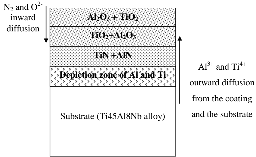
Figure 254 Final scale developed on TiAlN/CrN+Al 2 O 3 coated Ti45Al8Nb alloy in unaffected region at 1023 K for 5000 hours (edge of the sample)
