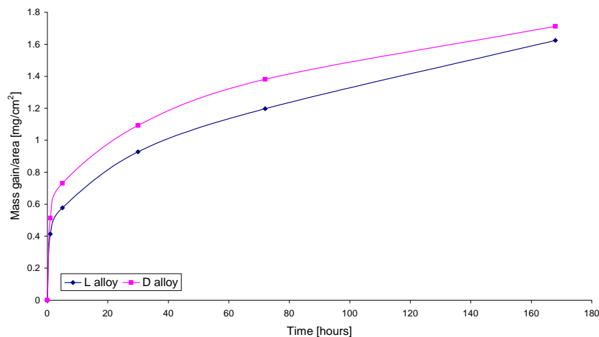
Figure 52 Mass gain of exposed samples (D – alloy and L - alloy) with k_p values (Ti46.6Al1.4Mn2Mo) to sulphidized/oxidised atmosphere at 1023 K [85]
