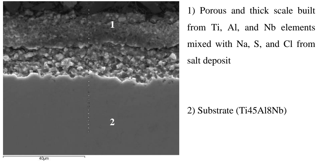
Figure 215 SEM cross section image (mag. 3000x) of CrAl2%YN coated Ti45Al8Nb after hot corrosion in salts mixture (20%NaCl/80%Na 2 SO 4 ) at 1023 K– affected region (edge of the sample)
