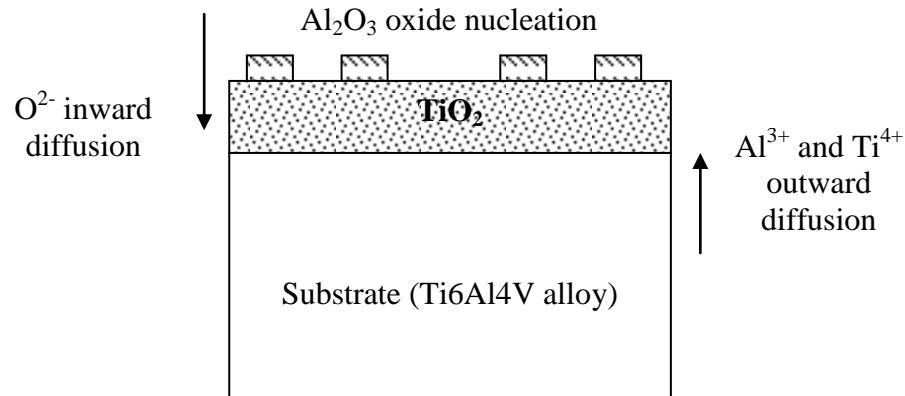
Figure 31b Nucleation of \text{Al}_2\text{O}_3 oxide and thickening of \text{TiO}_2 [54]
