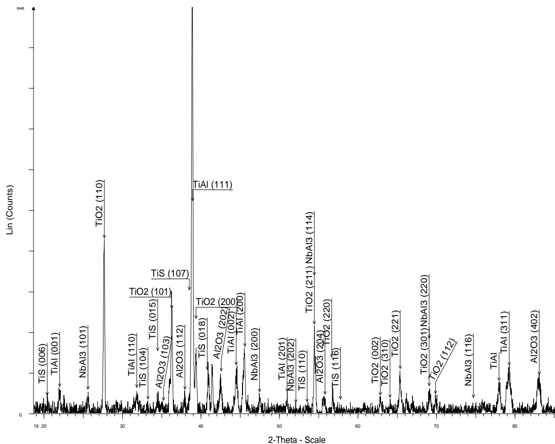
Figure 152 XRD pattern Ti45Al8Nb uncoated after 1000 hours sulphidation at 1023 K
