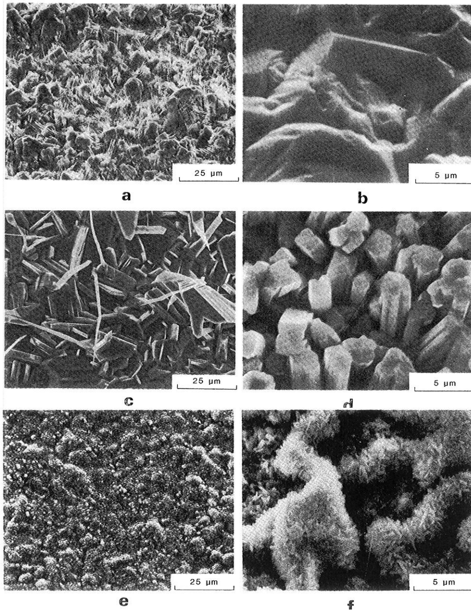
Figure 62 Scanning electron micrographs showing surface morphology of Ti and Ti6Al4V after exposure for 72 hours at 1023 K; a) Ti and b) Ti6Al4V in H 2 /H 2 O/H 2 S; c) Ti and d) Ti6Al4V in H 2 /H 2 O; e) Ti and f) Ti6Al4V in air [91]
