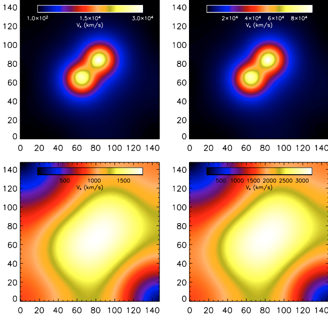
Fig. 4. Dynamic range of the Alfvén speed at 10 Mm ( top row ) and 60 Mm ( bottom row ) for two sets of free parameters (\rho_0, H) in (\text{cm}^{-3}, \text{Mm}) : (10^9, 25) , (10^8, 50) from left to right.
