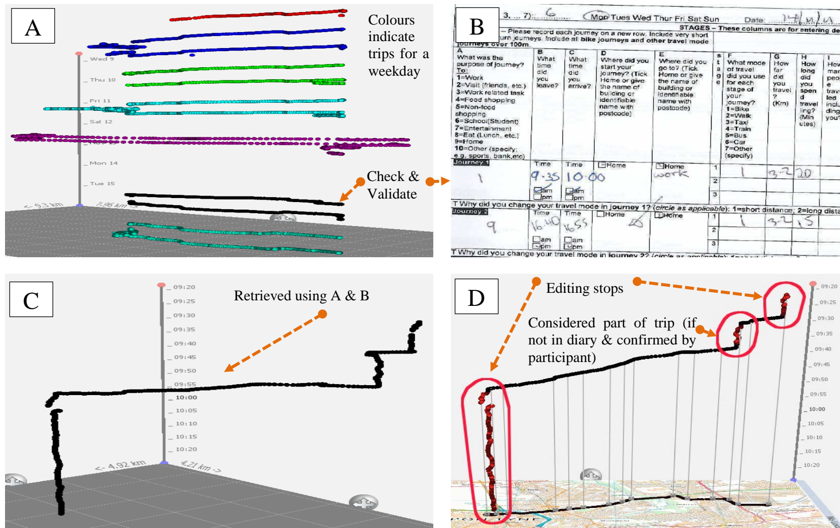
Figure 5-8: STC based data processing in four steps
