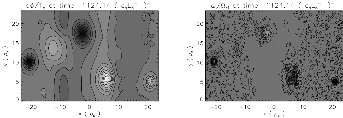
FIG. 13. The normalised potential e\phi/T_e and normalised vorticity \omega/\Omega_{ci} at 1124.14 characteristic time units for two parallel streams. The minimum and maximum values of e\phi/T_e are -2.3 \times 10^{-2} and 2.4 \times 10^{-2} , while the extrema for \omega/\Omega_{ci} are 0.18 and 0.2. Maximum is white and minimum is black in both plots. The negative vortex at x = -3\rho_s moves at speed 0.7 \max |v_\star| and the positive vortex at x = 6\rho_s moves at 1.2 \max |v_\star| , both in the negative y direction.
