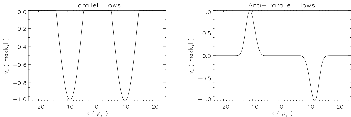
FIG. 12. Constant x profiles of diamagnetic velocity v_\star normalised to \max|v_\star| for two streams with a space between them. The characteristic time is (c_s L_n^{-1})^{-1} = 8.9 \times 10^{-6} \text{ s} for both parallel and anti-parallel streams.
