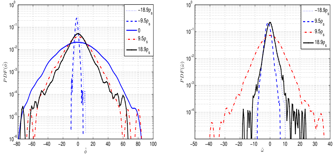
FIG. 5. Numerical PDFs along the x direction of the potential (graph on the left) and vorticity (graph on the right) time traces in the one stream case. The various x positions sampled are indicated by black vertical lines in Figure 4.
