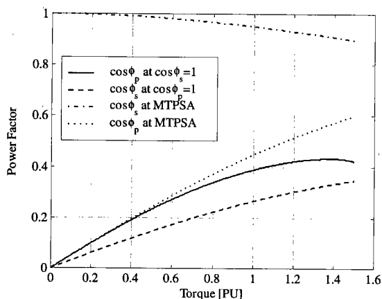
Fig. 11. Power factor performance for different control strategies
