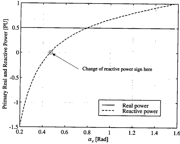
Fig. 6. Primary winding real ( P_{pn} ) and reactive ( Q_{pn} ) powers for T_n = 1
