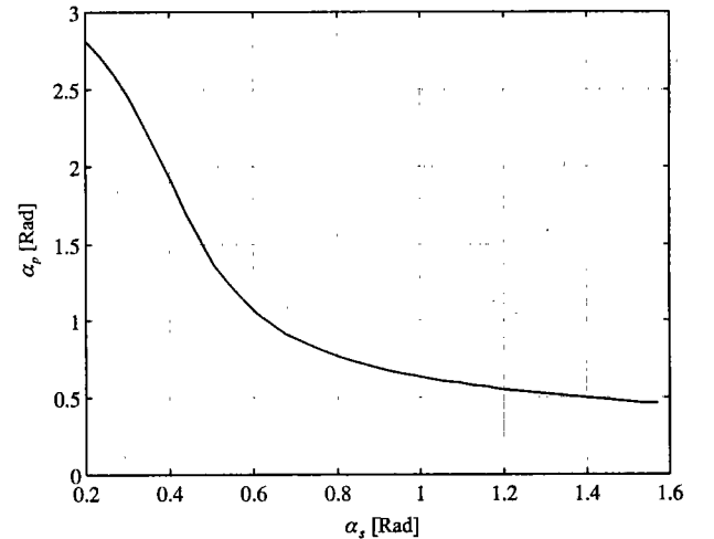
Fig. 5. The \alpha_p and \alpha_s angles for constant T_n = 1
