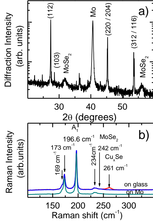
Figure 2 a) XRD pattern of a CZTSe film on Mo, b) Raman spectra of the CZTSe thin films on glass and Mo.
