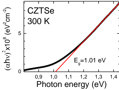
Figure 3 Optical absorption spectrum of CZTSe calculated at room temperature.
