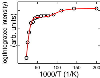
Figure 7 Temperature dependent quenching of the integrated intensity of the DAP peak.
