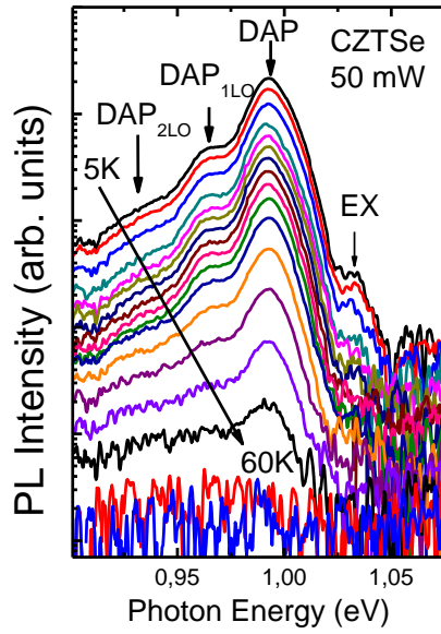
Figure 6 Temperature dependence of the PL spectra of the CZTSe film.
