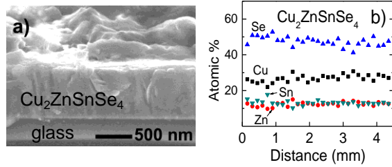
Figure 1 a) Cross sectional SEM micrograph of a CZTSe film on glass, b) WDX linescan.
