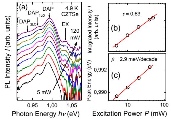
Figure 4 a) Excitation power dependence of the CZTSe PL spectra taken at 4.9 K, b) log/log dependence of the integrated intensity I on the excitation power P , c) dependence of the spectral position of the DAP peak on \log(P) .
