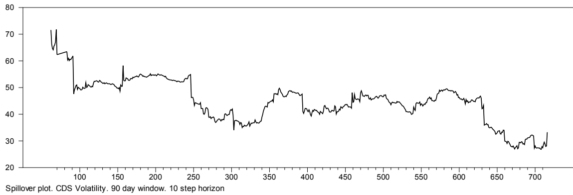
Fig. 2. Total CDS volatility spillovers plot
