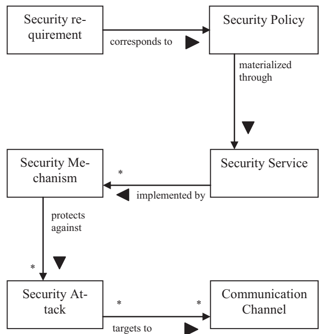
Fig 1: Security in distributed information system
