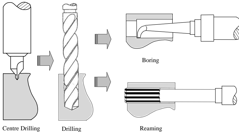
Figure 2 Hole producing processes and their relationships
