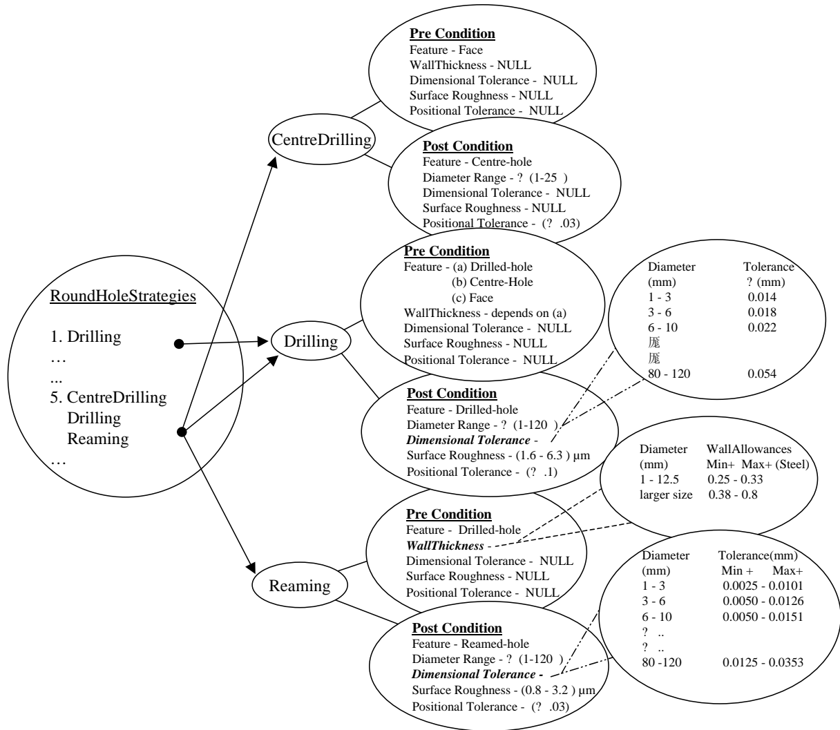
Figure 5 Example of manufacturing strategies link to ‘Pre’ and ‘Post’ conditions.
