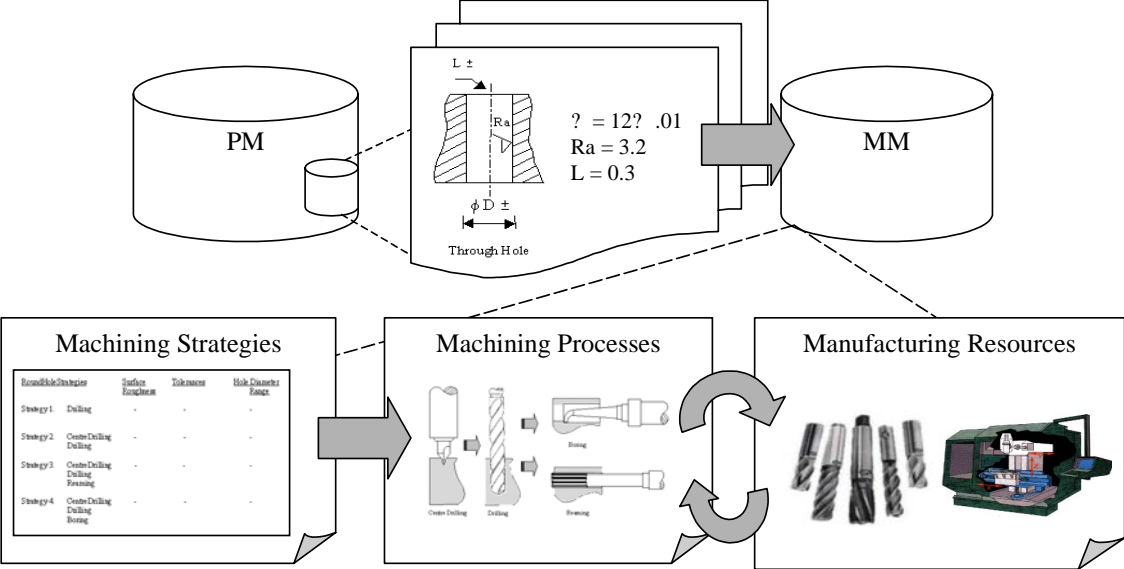
Figure 4 Relationships between product and manufacturing information
