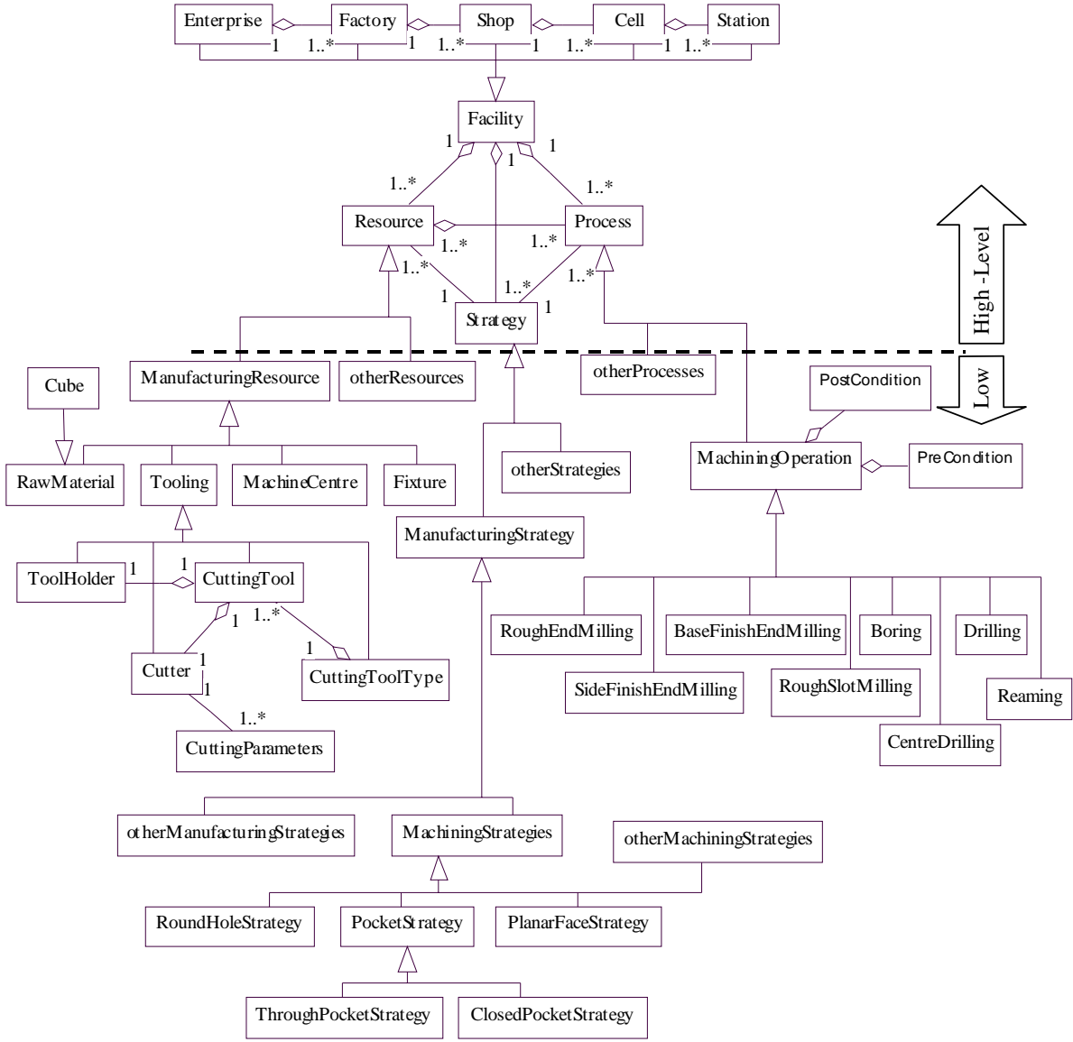
Figure 6 Manufacturing data model in UML representation
