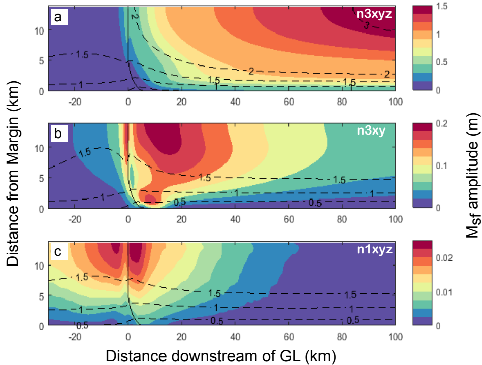
Figure 4. Plan view of M_{sf} amplitude in horizontal surface ice displacements, calculated with the full-Stokes viscoelastic model for the three experiments described in Sect. 5. Panel (a) shows experiment n3xyz, i.e. the standard case with n = 3 and bending all along the sidewall boundary. Panel (b) shows experiment n3xy in which the ice only bends at the x = 0 GL. Panel (c) shows the n1xyz experiment, for which n = 1 but with the same BCs as panel (a). Dashed black lines are contours of downstream mean surface ice velocity, and solid black lines show the GL position. Note the differences in colour scale between each panel.
