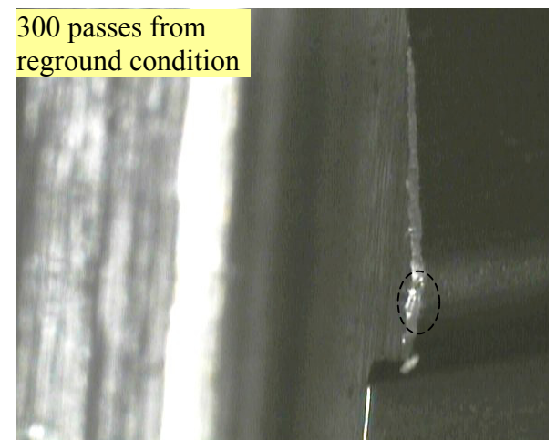
TiAlN coated teeth
