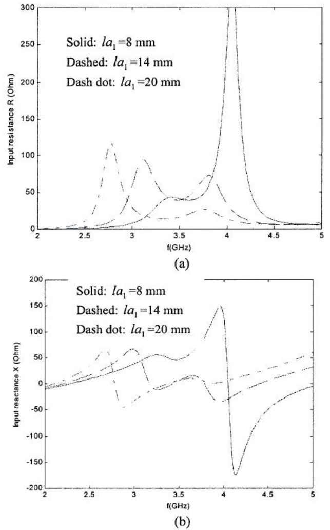
Fig. 4. Input impedance of the single-port antenna with different slot length la_1 . Other parameters: L = 29 mm, W = 30 mm, h_0 = 6.4 mm, la_2 = 2 mm, wa_1 = 1 mm, wa_2 = 4 mm, l_s = 5 mm, ds_2 = 14.5 mm. (a) Resistance R versus frequency f . (b) Reactance X versus frequency f .
