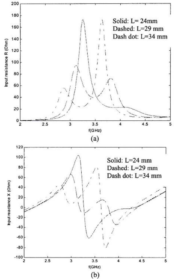
Fig. 2. Input impedance of the single-port antenna with different patch length L . Other parameters: W = 30 mm, h_0 = 6.4 mm, la_1 = 14 mm, la_2 = 2 mm, wa_1 = 1 mm, wa_2 = 4 mm, l_s = 5 mm, ds_2 = L/2 . (a) Resistance R versus frequency f . (b) Reactance X versus frequency f .
