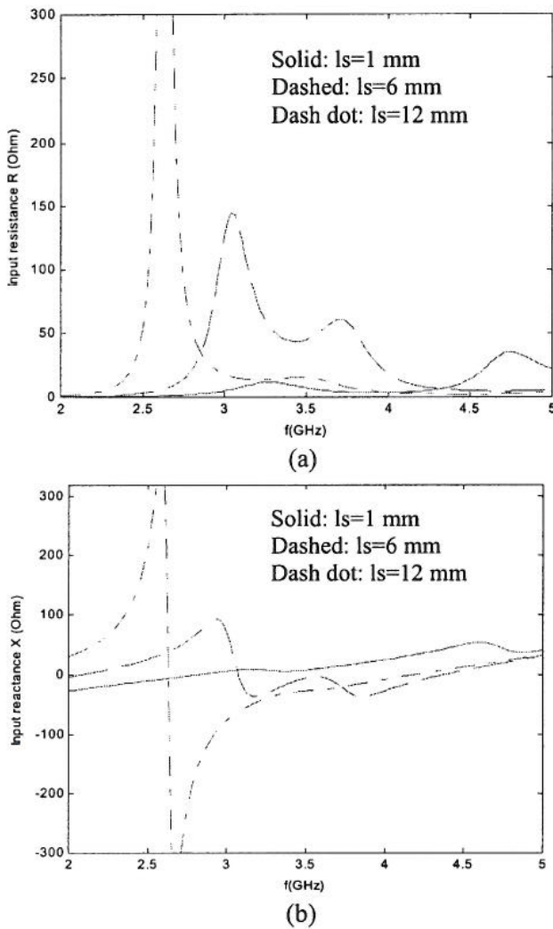
Fig. 3. Input impedance of the single-port antenna with different open stub length l_s . Other parameters: L = 29 mm, W = 30 mm, h_0 = 6.4 mm, la_1 = 14 mm, la_2 = 2 mm, wa_1 = 1 mm, wa_2 = 4 mm, ds_2 = 14.5 mm. (a) Resistance R versus frequency f . (b) Reactance X versus frequency f .
