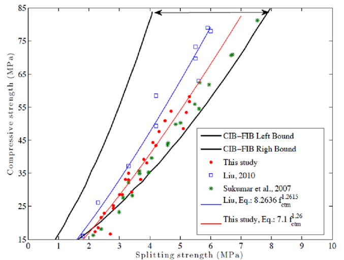
Fig. 3. Compressive strength vs splitting tensile strength of SCC with fly ash and blended aggregate in comparison with SCC with only fly ash.
