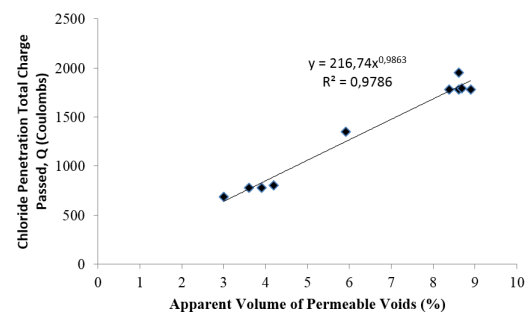
Fig. 9. Apparent volume of permeable voids vs. chloride penetration
