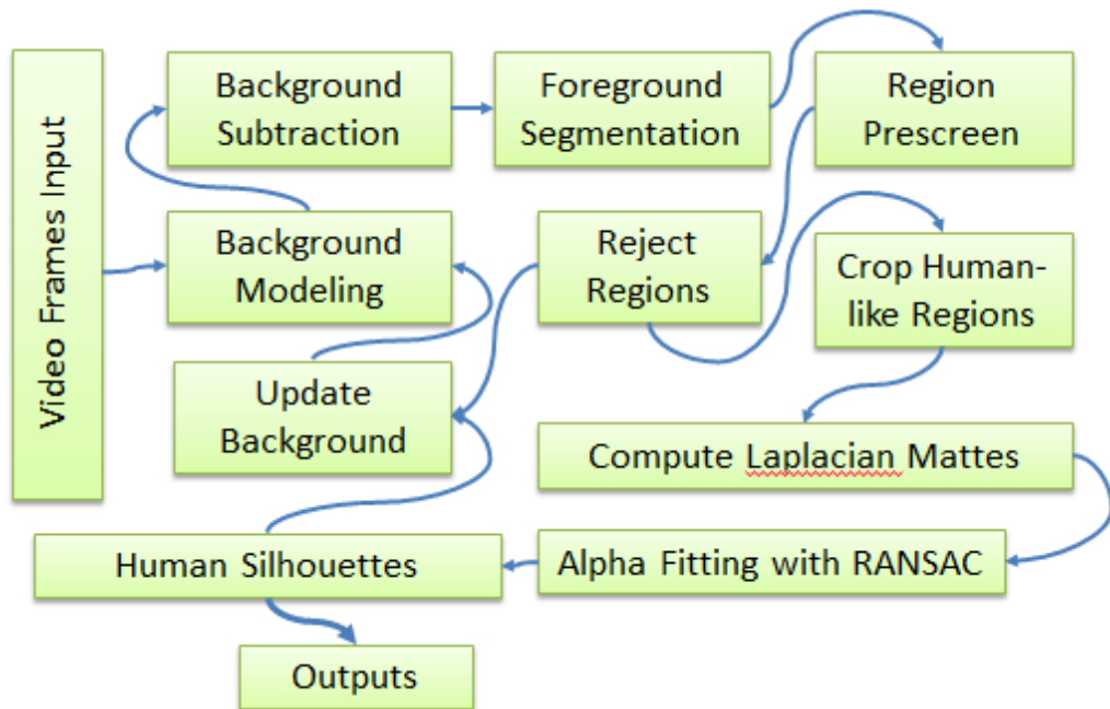
Figure 0.1 Schematic view of our Laplacian fitting algorithm.
