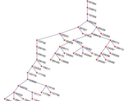
Fig. 3: Low voltage rural distribution feeder.
