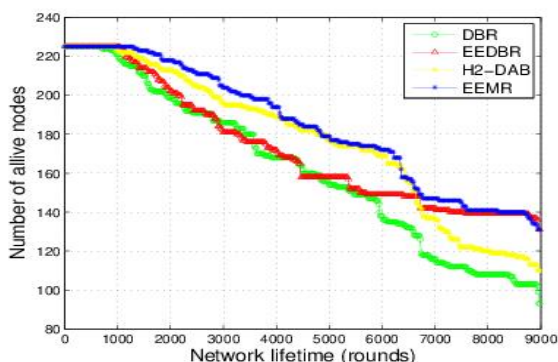
Fig. 6: Number of Alive Nodes vs Network Life Time
