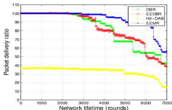
Fig. 7: Packet Delivery Ratio vs Network Life Time
