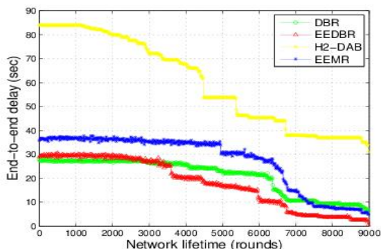
Fig. 5: End to End Delay vs Network Life Time
