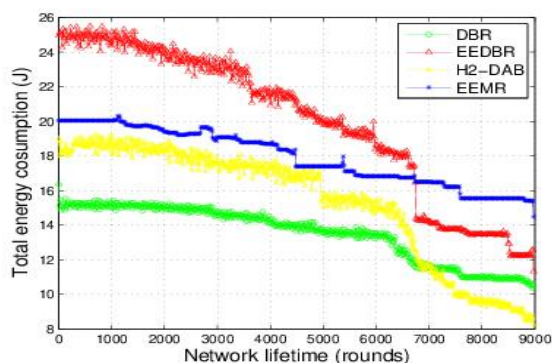
Fig. 8: Total Energy Consumption vs Network Life Time
