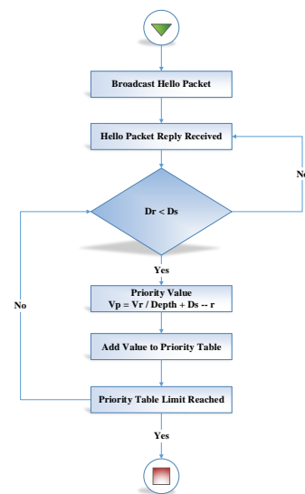
Fig. 4: Priority Table Creation Flow Chart
