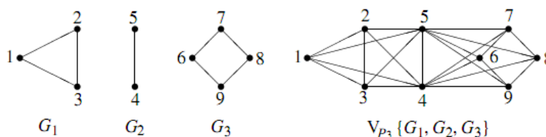
Figure 1. The joined union H = P_3[G_1, G_2, G_3] .
