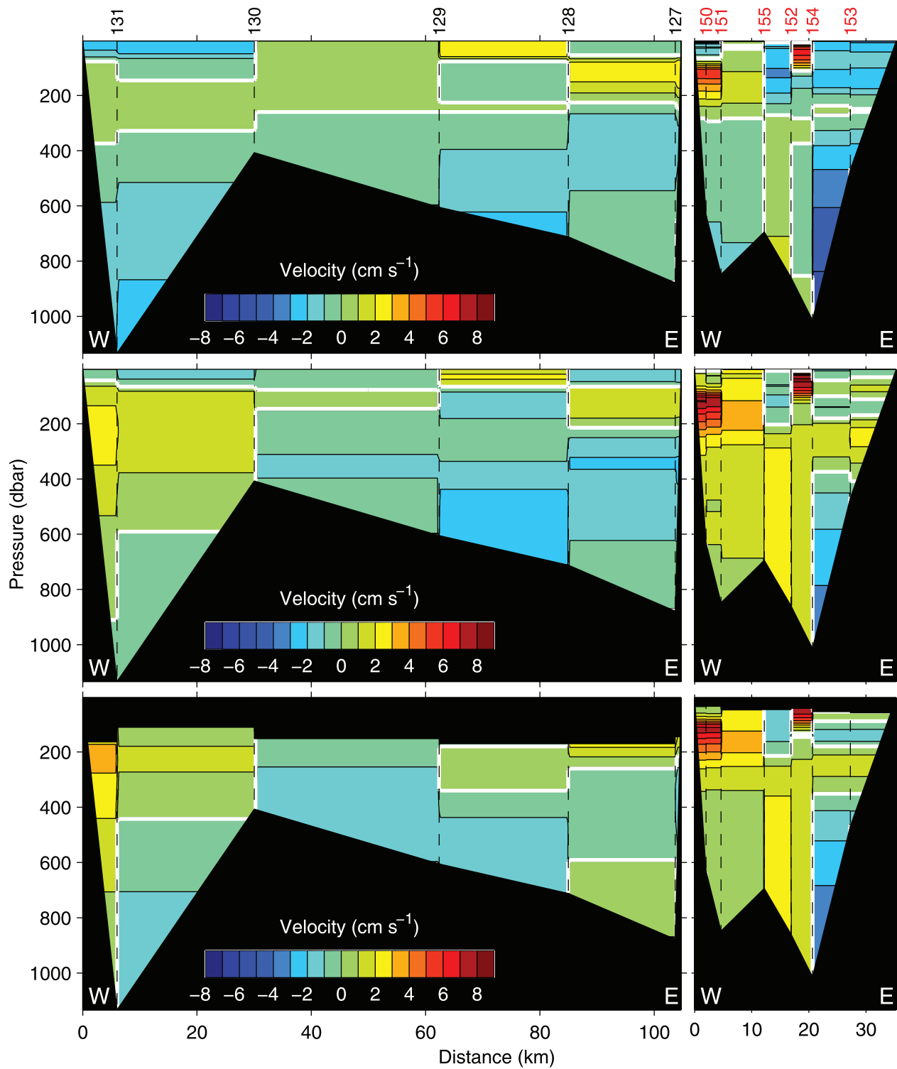
Figure 8. (top) Initial and (middle and bottom) final velocities calculated at the (left) southern and (right) northern ice fronts. Positive values indicate flow out of the cavity (into the page), and the bold white line corresponds to zero velocity. The initial velocities were set to have a level of zero motion along the 5 per mille meltwater fraction contour. The final velocities represent a minimal adjustment to the initial values that will permit overall balanced tracer budgets over the full water column (middle) and over the partial water column where the meltwater fraction calculations are unaffected by atmospheric interaction (bottom). In the latter case the part of the water column excluded from the consideration is shaded black.
