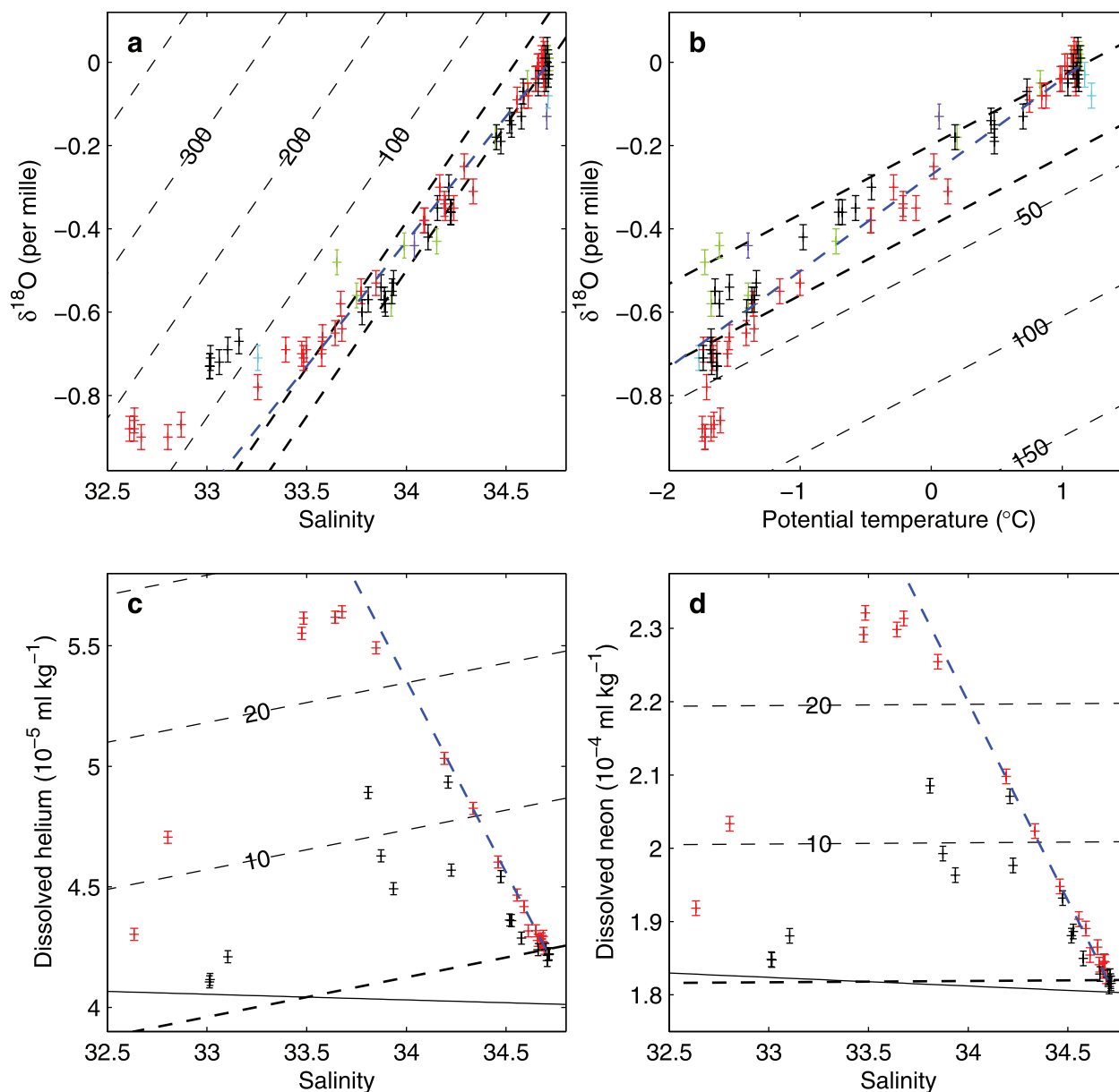
Figure 7. (a) The \delta^{18}\text{O}/\text{S} , (b) \delta^{18}\text{O}/\theta , (c) \text{He}/\text{S} , and (d) \text{Ne}/\text{S} data obtained at the stations marked in Figure 1. Color coding of the individual stations corresponds to that indicated in Figure 1. In all cases the numbered, light dashed lines are contours of meltwater fraction (per mille), while the bold dashed lines indicate the theoretical upper bound on the melt fraction and the CDW/WW trend used to define the zero melt fraction contour. The blue dashed lines indicate the CDW/meltwater mixing trends. The near-horizontal solid lines in Figures 7c and 7d indicate saturation concentrations for water at the surface freezing point.
