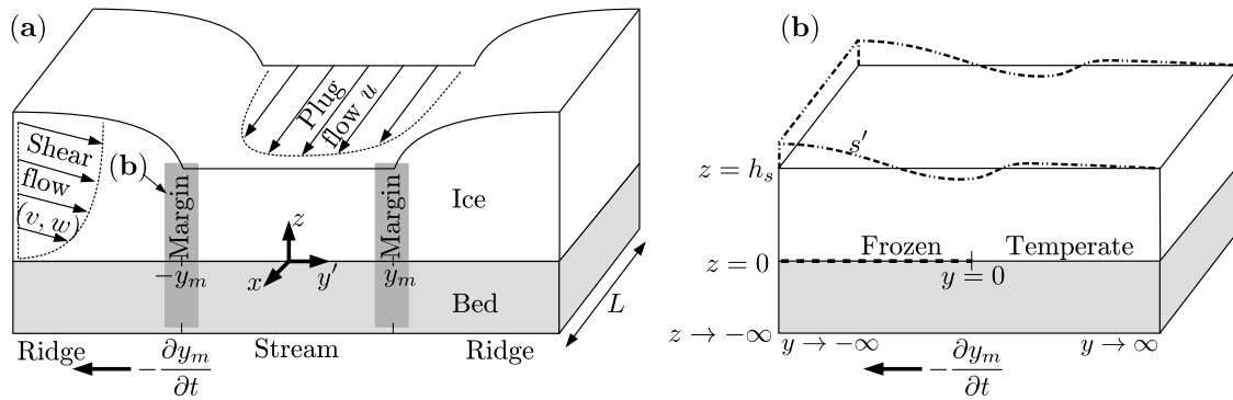
Figure 1. Panel (a) shows large-scale model geometry: we assume an ice stream flowing in positive x direction. At its sides, the ice stream is bordered by slowly moving ice ridges. Panel (b) shows boundary layer geometry, which moves at the rate v_m = \partial y_m / \partial t through the ice stream/ridge geometry shown in panel (a).
