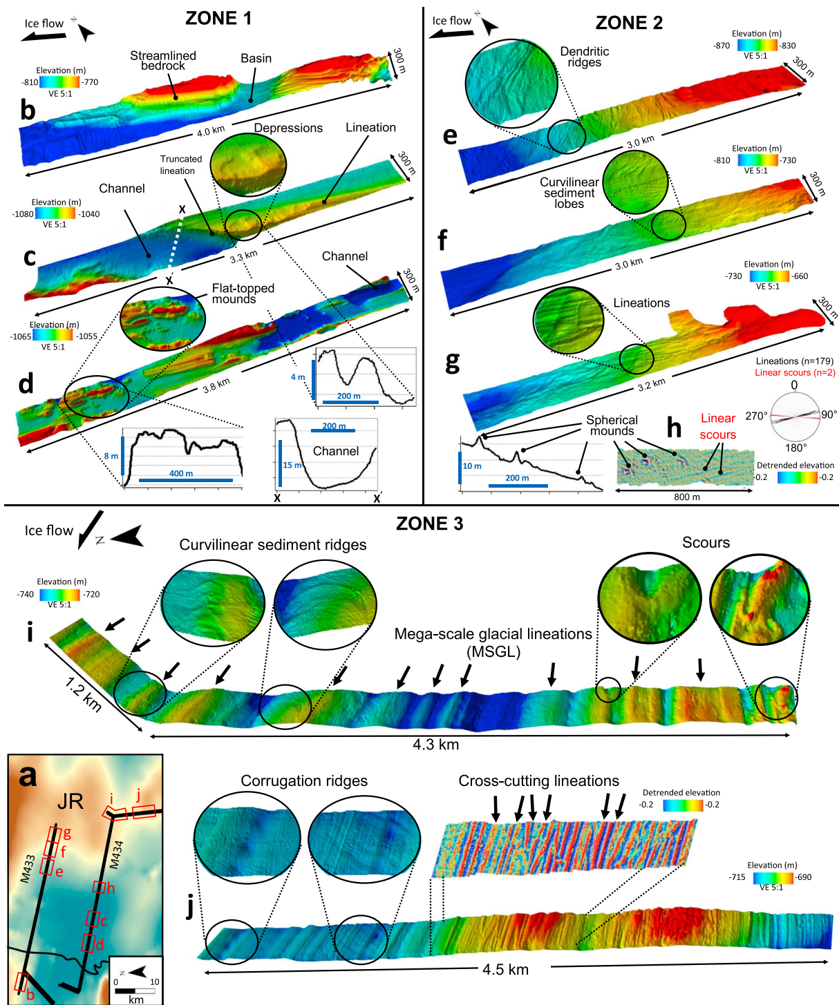
Figure 3. Three-dimensional surfaces of multibeam seafloor bathymetry. (a) Inset map showing the locations of Figures 3b–3j. Multibeam surface imagery of seafloor topography and extracted topographic profiles in (b–d) Zone 1, (e–h) Zone 2, and (i and j) Zone 3. Location of Figure 3h is shown in the inset map and Figure 2e. Rose diagram next to Figure 3h shows the azimuth of lineations sampled from Zones 1–3 compared to linear scours in Figure 3h.
