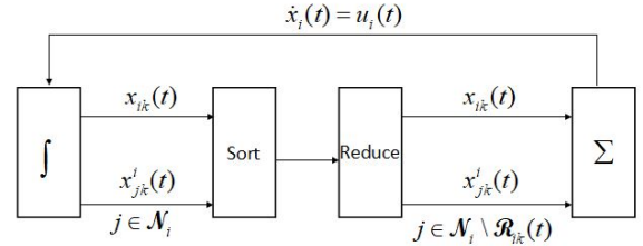
Fig. 1. Data flow model of MSR algorithm for agent i .
