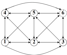
Fig. 3. A directed graph G with N = 6 agents.
