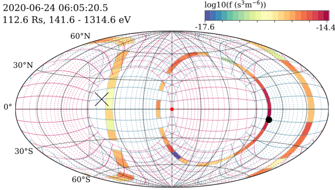
Fig. 2. A sky map representation of the combined EAS FOV in the spacecraft (SC) reference frame. The centre of the plot is aligned with the X-axis, 90^\circ in longitude with the Y-axis, and latitude corresponds to the Z-axis. The angular bins are shown in blue for EAS 1 and in red for EAS 2. Two elevation bins of the EAS 1 head are filled with data obtained during one scan in the instrument Burst Mode (BM). The magnetic field direction is marked with a black dot (+ \mathbf{B} ) and a black cross ( -\mathbf{B} ).
