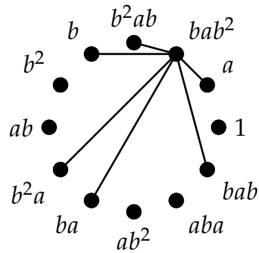
Figure 4. \Delta_{H_2, A_4}^{b^2ab} .
