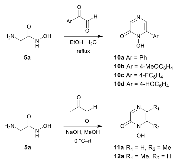
Scheme 2. Synthesis of 1-hydroxypyrazin-2(1H)-ones 10a–10d , 11a and 12a .
