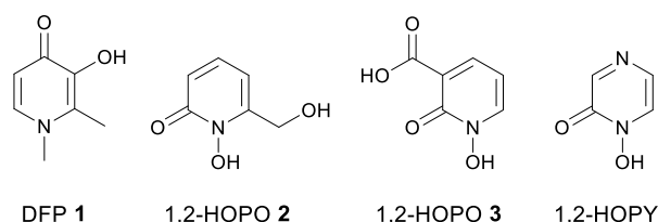
Figure 1. Structures of deferiprone (DFP 1 ), and 1-hydroxypyridin-2(1H)-ones 2 and 3 .
