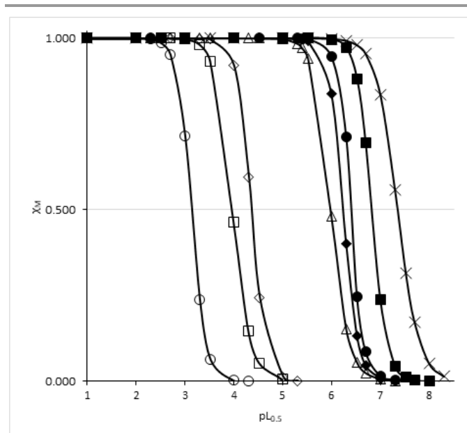
Figure 4. Sequestration diagrams towards \text{Fe}^{3+} at pH = 7.4 of ligands 11a (○), 10a (□), 6a (◇), 6c (△), 6d (×) and previously studied ligands 2 (◆), 3 (●) and DFP 1 (■) and. [\text{Fe}^{3+}] = 10^{-9} \text{ M} , T = 25.0^\circ \text{C} , I = 0.1 \text{ M} ( \text{NaClO}_4 ).
