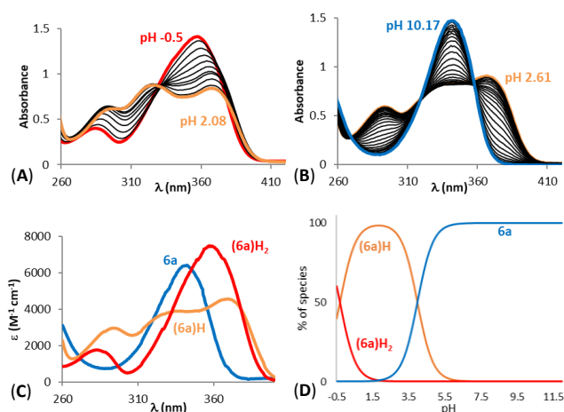
Figure 2. Spectrophotometric titrations vs pH of ligand 6a between (A) -0.5 < \text{pH} < 2.08 (batch titration, [\text{6a}] = 2.57 \times 10^{-4} \text{ M} ) and (B) 2.61 < \text{pH} < 10.17 (direct titration, [\text{6a}] = 2.55 \times 10^{-4} \text{ M} ). (C) Electronic spectra and (D) distribution curves ( [\text{6a}] = 1.54 \times 10^{-4} \text{ M} ) of the protonated species of ligand 6a . Solvent: H 2 O, I = 0.1 M (NaClO 4 ), T = 25.0 °C.
