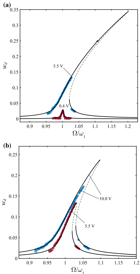
Fig. 2 Frequency responses of the MEMS resonator at V_{DC} = 5 V, and different AC voltages (denoted on the curves). Circles: experimental data; lines: theoretical predictions using the linear damping model with a coefficient of a c_d^{(1)} = 0.107 calibrated based on the experimental results for V_{AC} = 0.4 V and b c_d^{(1)} = 0.305 calibrated based on the experimental results for V_{AC} = 5.5 V
