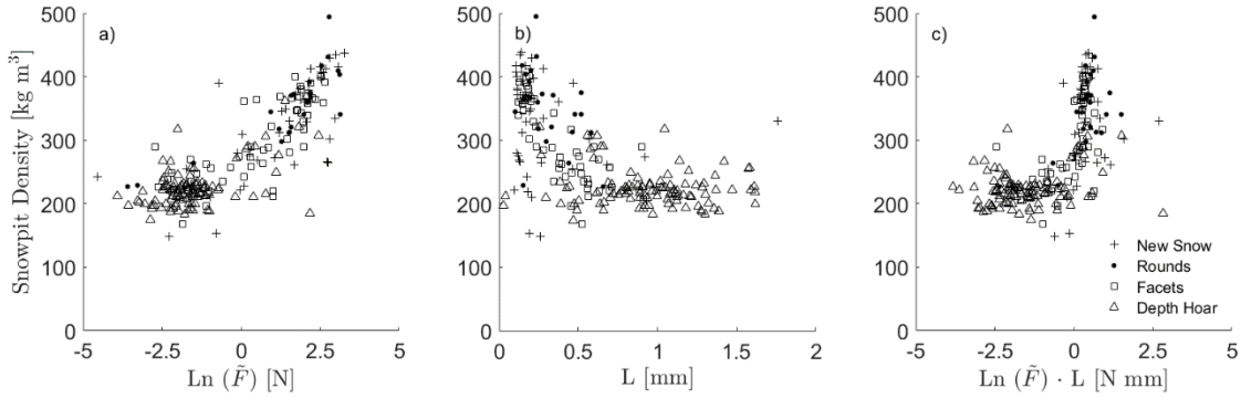
Figure A2: Relationships between the snowpit densities and SMP microstructural metrics from the paired profiles in the recalibration dataset, after Figure 5 of King et al. (2020b).
