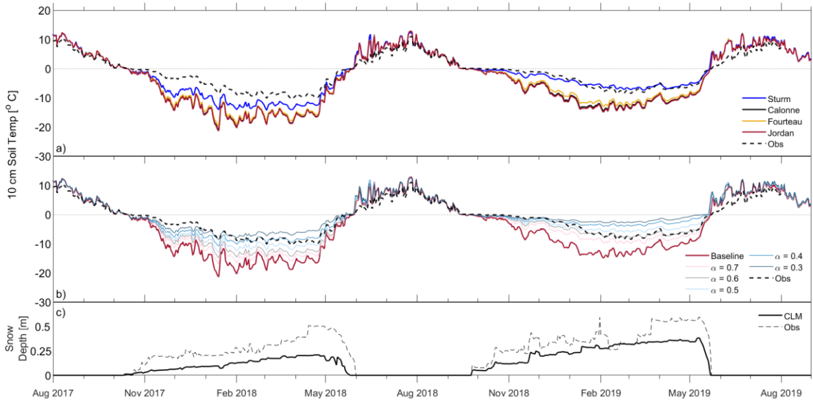
845 Figure 7: a) Simulated 10cm soil temperature timeseries using the 4 different parameterisations of snow thermal conductivity compared to field measurements, b) Timeseries of 10cm soil temperatures when using different values of the correction factor \alpha compared to field measurements, c) Observed and simulated snow depths for the same time period.
