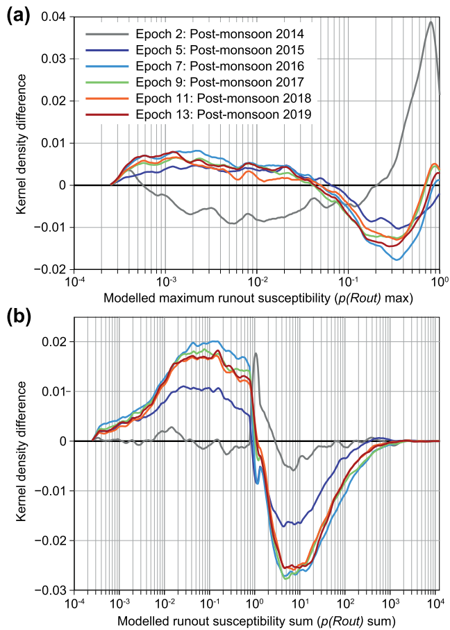
FIGURE 4 Kernel density estimates of the distributions of (a) maximum per-cell runout susceptibility ( p(Rout)_{max} ) and (b) the per-cell sum of all runout susceptibilities ( p(Rout)_{sum} ), expressed as the difference between each distribution and the coseismic distribution in Epoch 4 (black line). Positive values represent a greater number of cells with corresponding value of p(Rout) , negative value represent a smaller number of cells relative to Epoch 4.
