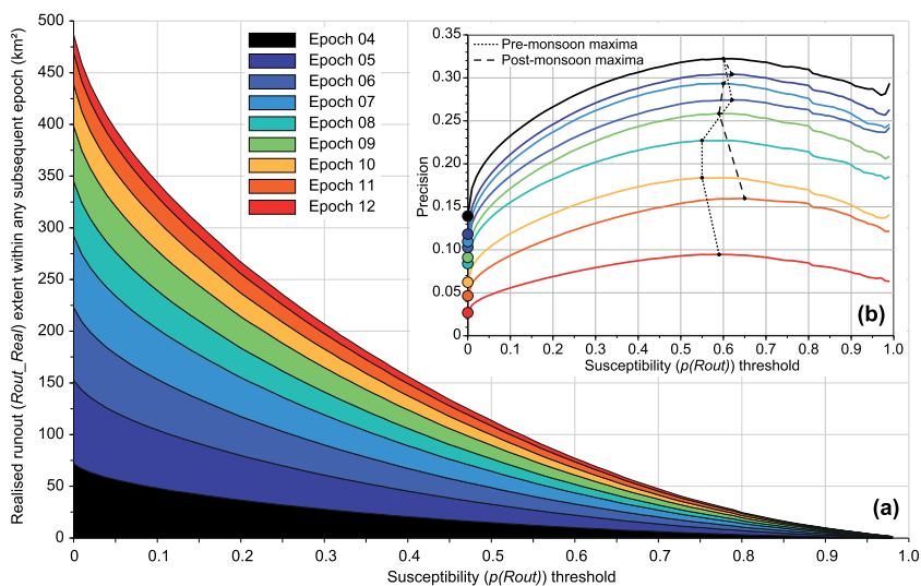
FIGURE 7 (a) Extent of modelled runout in each of the mapping epochs that was realized by landslide occurrence within any subsequent epoch ( Rout\_Real ), differentiated by susceptibility ( p(Rout) ) threshold. Note: The realization area data on the y-axis are stacked. (b) Model precision by epoch, defined as the realized runout area ( Rout\_Real ) as a fraction of the total coseismic runout area ( Rout\_Mod ), again differentiated by susceptibility ( p(Rout) ) threshold. For all epochs, the model achieves maximum precision at a p(Rout) threshold of 0.55–0.65; these points are connected for reference to show their evolution in time for both pre- and post-monsoon inventories. Coloured dots on the y-axis indicate the proportion of all Rout\_Mod that was realized by the end of the study for each mapping epoch.
