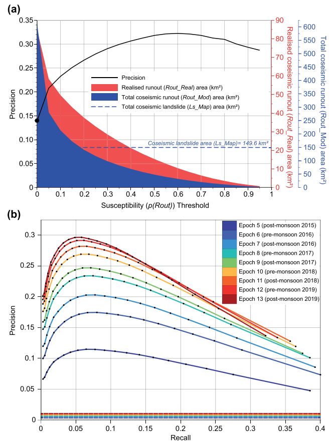
FIGURE 5 (a) Area of modelled coseismic runout ( Rout_{Mod} ; blue) and area of modelled coseismic runout that was realized by landslide occurrence within any post-EQ epoch ( Rout_{Real} ; red), as a function of modelled susceptibility p(Rout) threshold. The black line shows the model precision, defined as the realized runout area ( Rout_{Real} ) as a fraction of the total coseismic runout area ( Rout_{Mod} ), again as a function of susceptibility ( p(Rout) threshold). The maximum model precision occurs at a p(Rout) threshold of 0.6. Black dot on the y-axis indicates that 14% of all coseismic Rout_{Mod} was realized by the end of the study. (b) Precision-recall curves for each of the post-seismic epochs, based on modelling of runout from coseismic (Epoch 4) landslides and comparison with subsequent mapped landslide inventories (Epochs 5–13). Each curve is calculated based on the cumulative extent of post-seismic landsliding that occurred up until that epoch. Black dots along the curve represent the susceptibility thresholds, increasing in 0.05 intervals from zero. Horizontal dashed lines towards the base of the y-axis show the no skill values for a random classifier from each epoch; note that the precision depends upon the number of positive values, and so varies between epochs.
