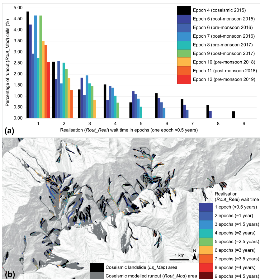
FIGURE 6 (a) Distribution of runout realization wait times for all coseismic and post-seismic epochs. Realization wait times are defined here as the time between when a cell is first included within a modelled runout area for a given epoch ( Rout_Mod ), and when it first intersected a mapped landslide polygon ( Rout_Real ). Note that longer wait times can only be determined for the earlier epochs due to the brevity of our inventory data. (b) Map showing an example of per-cell realization wait times associated with the modelled coseismic runout for an area of Dolakha district. The spatial extent of this map is shown on Figure 1 for reference.
