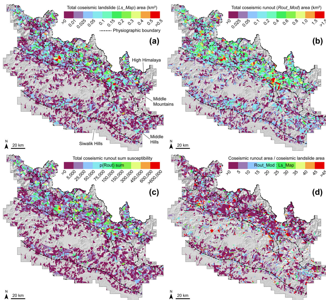
FIGURE 8 Spatial distribution of key runout metrics aggregated by individual slope unit. (a) Total coseismic landslide ( Ls\_Map ) area; (b) total modelled coseismic runout ( Rout\_Mod ) area; (c) summed susceptibilities ( p(Rout) ) of coseismic runout; (d) ratio of coseismic runout area to landslide area ( Rout\_Mod:Ls\_Map ). Dashed black lines represent the major physiographic boundaries within the study area.
