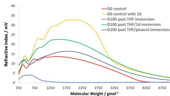
Fig. 10 GPC analysis of the solutions from 1d and pinacol chemical recycling methodologies (according to Fig. 7) vs. D0 controls (with and without 1d ).
