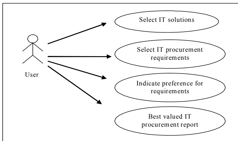
Figure 7: Use-case diagram
