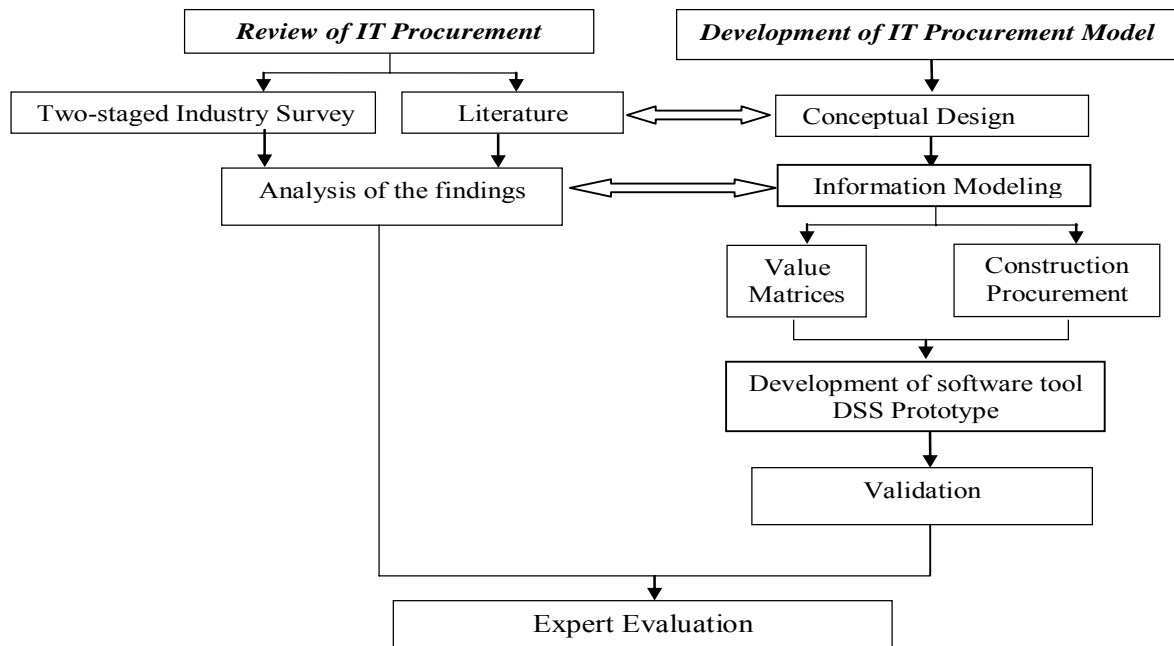
Figure 1 Research Methodology
