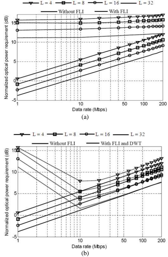
Fig. 4: The NOPR versus the data rates for 4, 8, 16 and 32 DH-PIM 1 with and without the FLI: (a) without DWT denoising and (b) with DWT denoising
