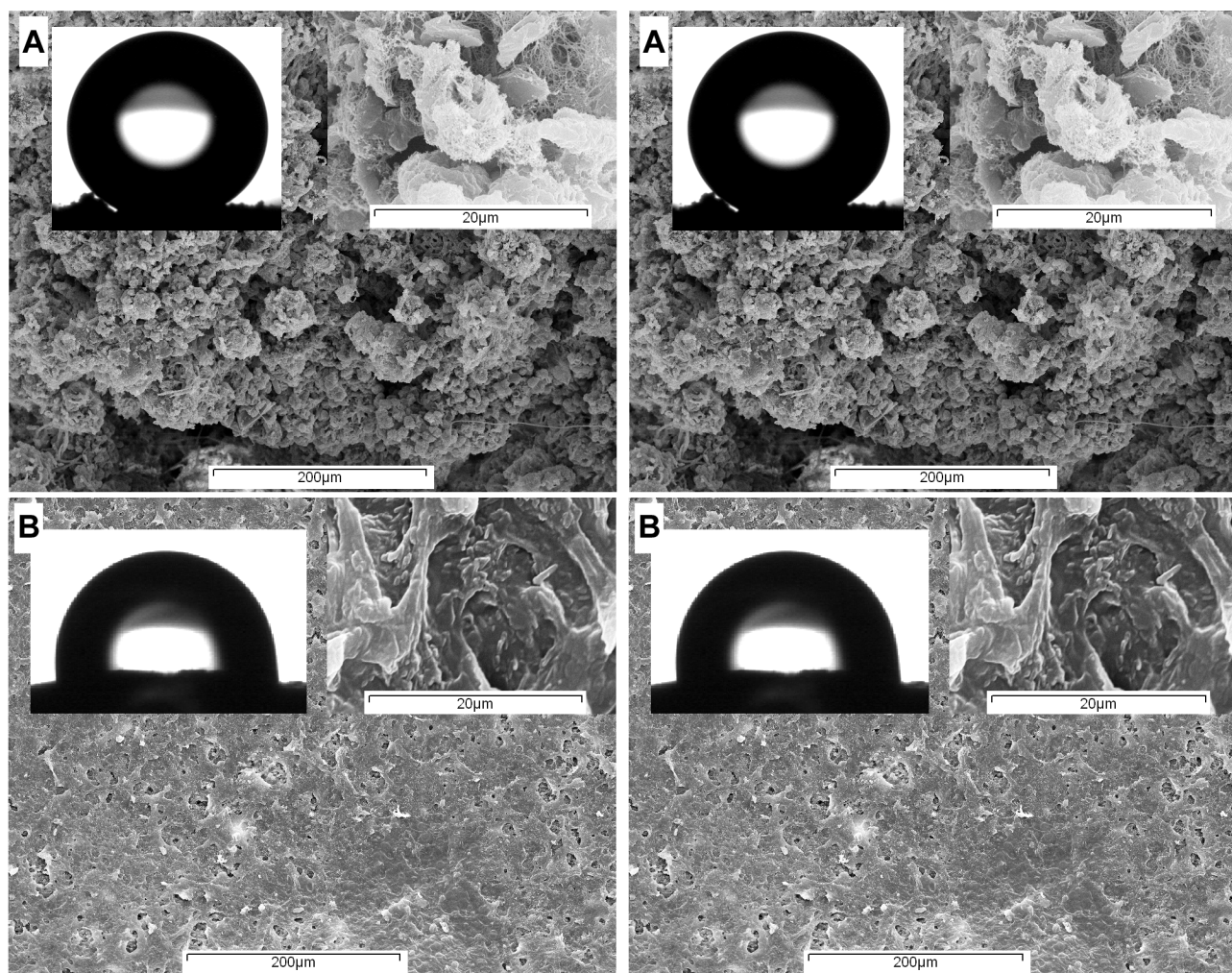
Figure 2. (A) main and inset right electron micrographs of Lecanora conizaeoides showing high roughness with photograph of water drop inset left, contact angle 155\pm4^\circ . (B) Main and inset right electron micrographs of a lichen, Flavoparmelia caperata ( Parmelia spp), and inset left a photograph of a drop of water on its surface, contact angle 89\pm4^\circ . SEM scale bars 200 \mu\text{m} (outer pictures) and 20 \mu\text{m} (insets).
