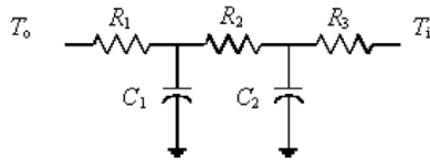
Figure 1: 2nd order lumped parameter construction element
