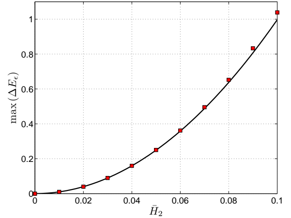
FIG. 5: (Color online) Maximum value of the relative energy \Delta E_\epsilon of the perturbed DW as a function of the amplitude of the transverse applied field, \bar{H}_2 . Numerically computed values are represented by (red) squares. The (black) solid curve is a parabola, \max(\Delta E_\epsilon) = C_H \bar{H}_2^2 with C_H = 99.6586 , fitted by the method of least squares through the data points with \bar{H}_2 \leq 0.04 .
